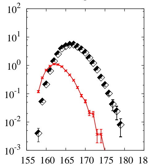
^{208}\text{Pb}(p,x)\text{Hf}
