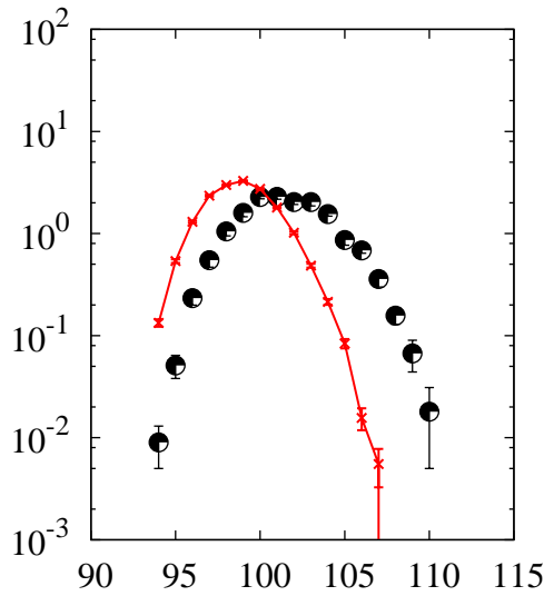
^{208}\text{Pb}(p,x)\text{Ru}
