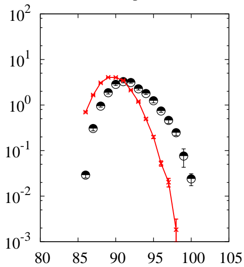
^{208}\text{Pb}(p,x)\text{Zr}
