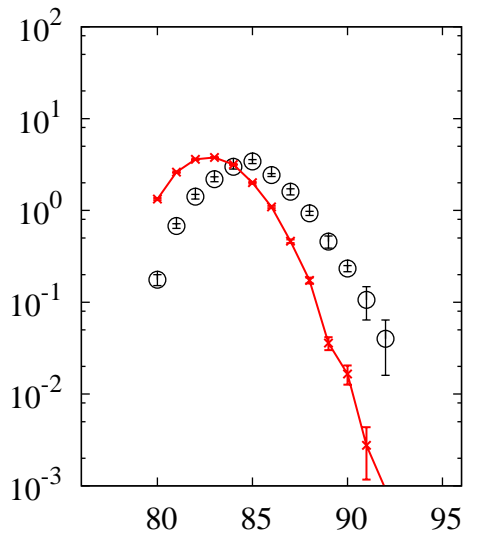
^{208}\text{Pb}(p,x)\text{Rb}
