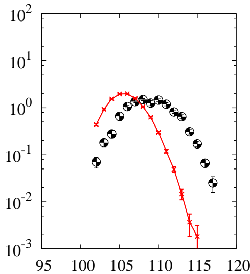
^{208}\text{Pb}(p,x)\text{Ag}
