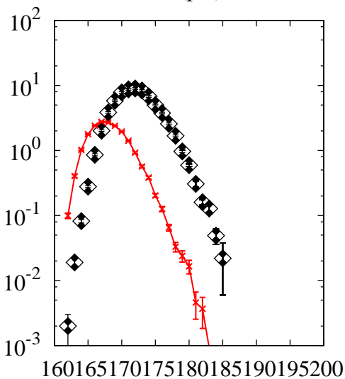
^{208}\text{Pb}(p,x)\text{W}
