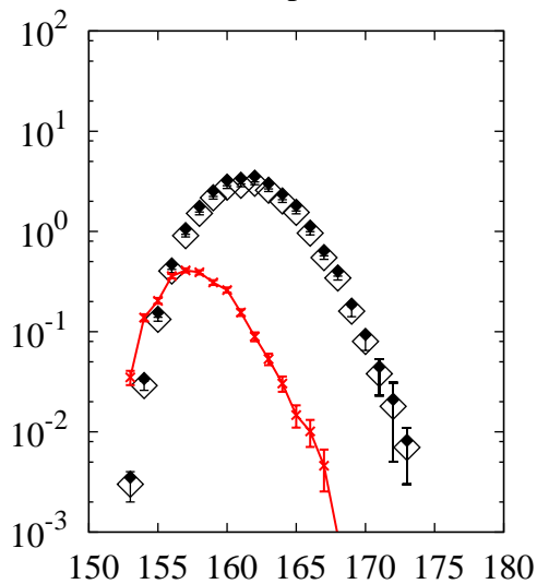
^{208}\text{Pb}(p,x)\text{Yb}
