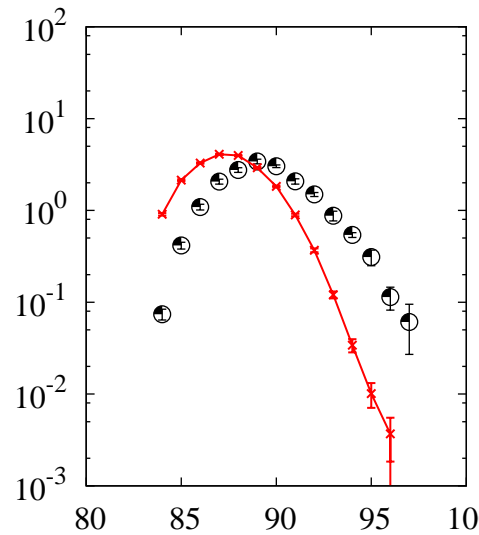
^{208}\text{Pb}(p,x)\text{Y}
