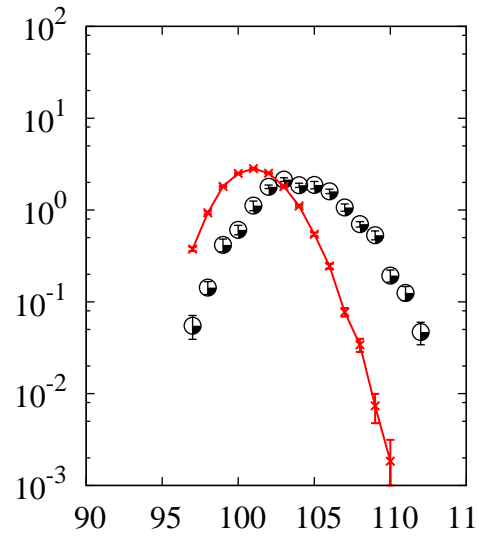
^{208}\text{Pb}(p,x)\text{Rh}
