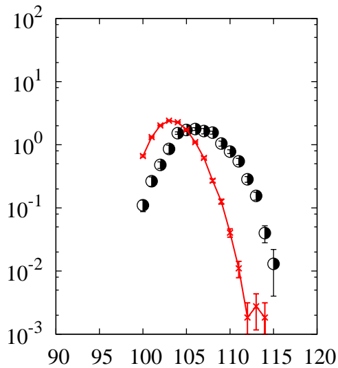
^{208}\text{Pb}(p,x)\text{Pd}
