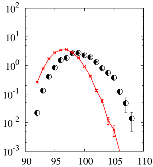
^{208}\text{Pb}(p,x)\text{Tc}
