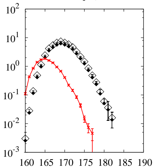
^{208}\text{Pb}(p,x)\text{Ta}
