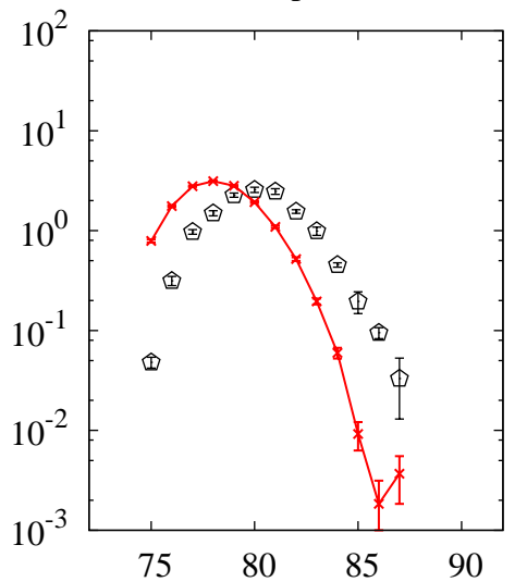
^{208}\text{Pb}(p,x)\text{Br}
