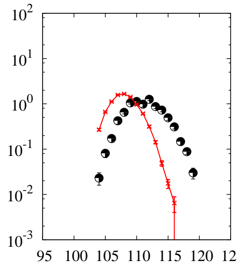
^{208}\text{Pb}(p,x)\text{Cd}
