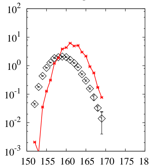
^{208}\text{Pb}(p,x)\text{Tm}
