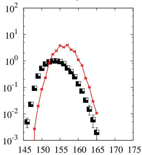
^{208}\text{Pb}(p,x)\text{Ho}
