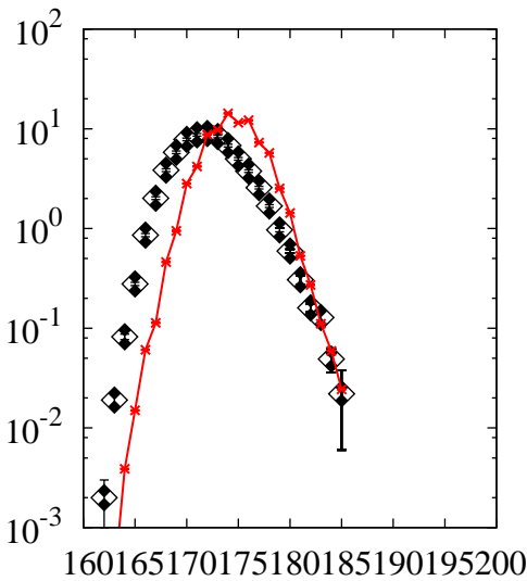
^{208}\text{Pb}(p,x)\text{W}
