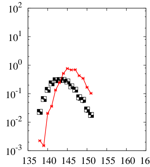
^{208}\text{Pb}(p,x)\text{Eu}
