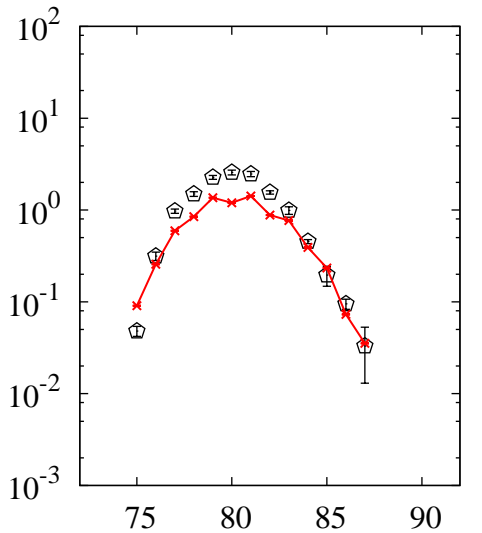
^{208}\text{Pb}(p,x)\text{Br}
