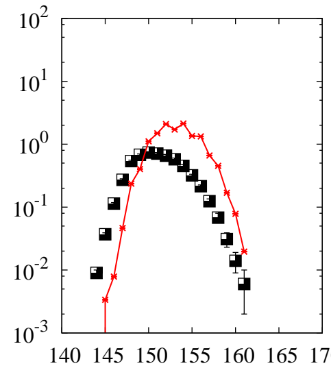
^{208}\text{Pb}(p,x)\text{Dy}
