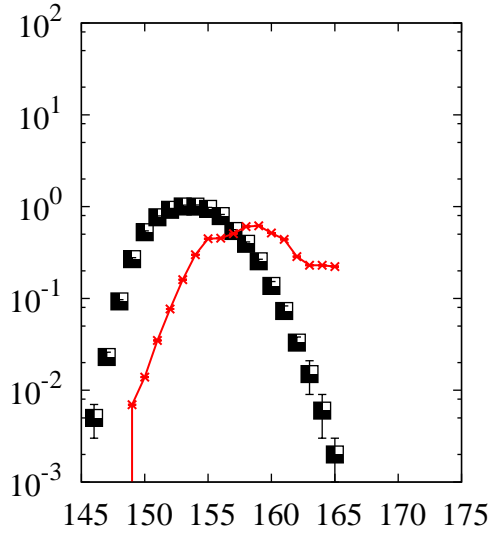
^{208}\text{Pb}(p,x)\text{Ho}
