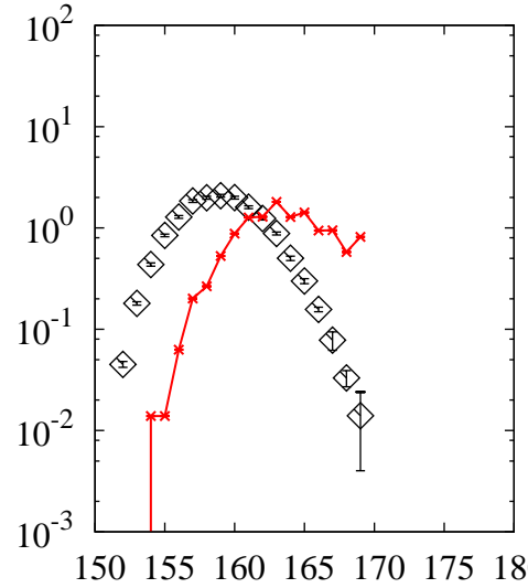
^{208}\text{Pb}(p,x)\text{Tm}
