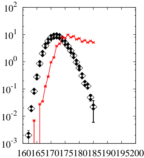
^{208}\text{Pb}(p,x)\text{W}
