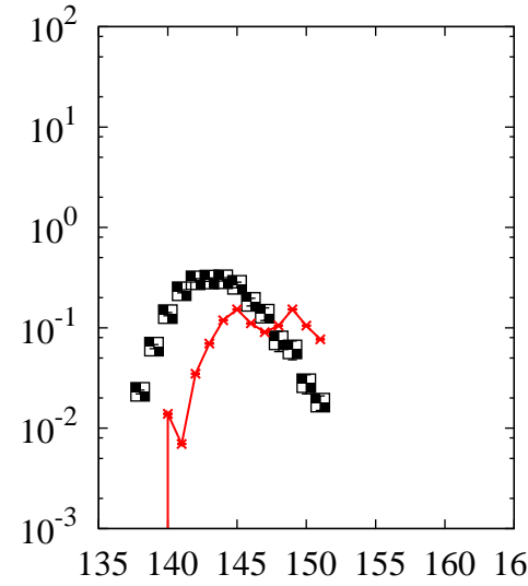
^{208}\text{Pb}(p,x)\text{Eu}
