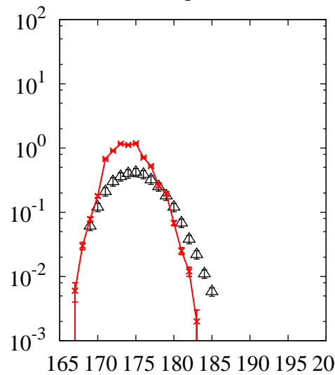
^{238}\text{U}(p,x)\text{Re}
