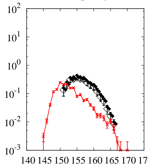
^{238}\text{U}(p,x)\text{Dy}
