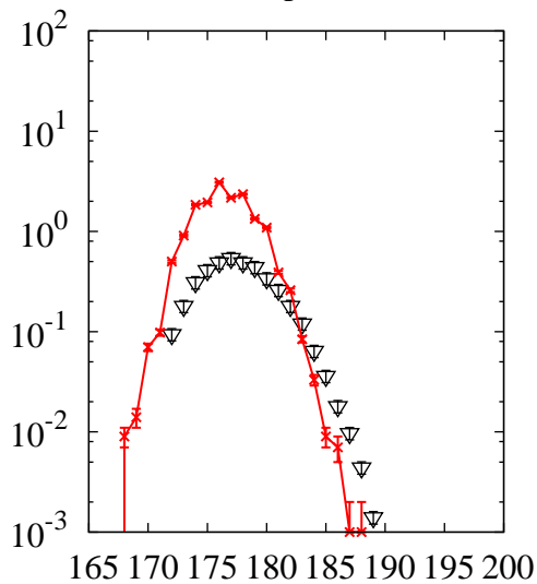
^{238}\text{U}(p,x)\text{Os}
