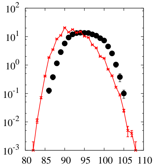
^{238}\text{U}(p,x)\text{Zr}
