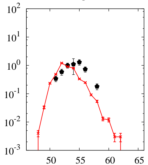
^{238}\text{U}(p,x)\text{Cr}
