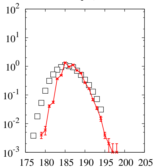
^{238}\text{U}(p,x)\text{Au}
