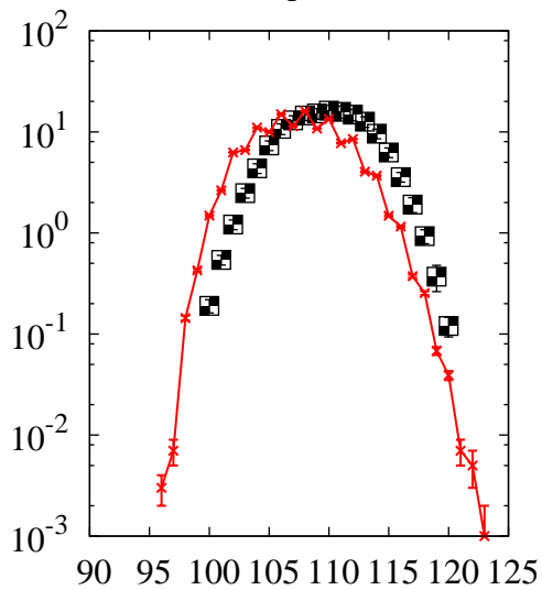
^{238}\text{U}(p,x)\text{Pd}
