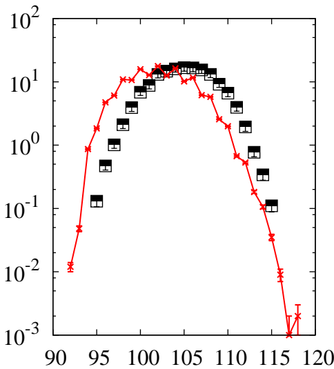
^{238}\text{U}(p,x)\text{Ru}
