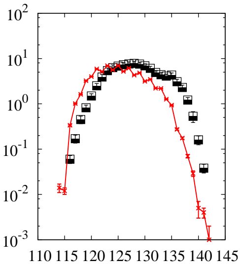
^{238}\text{U}(p,x)\text{I}
