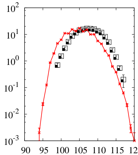
^{238}\text{U}(p,x)\text{Rh}
