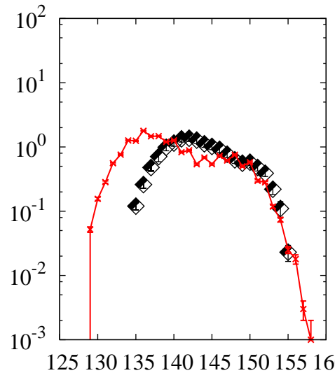
^{238}\text{U}(p,x)\text{Nd}
