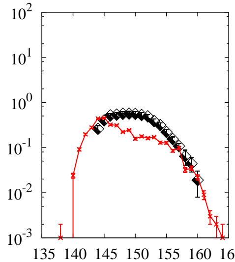
^{238}\text{U}(p,x)\text{Eu}
