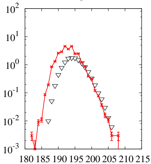
^{238}\text{U}(p,x)\text{Pb}
