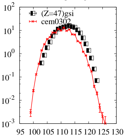
^{238}\text{U}(p,x)\text{Ag}
