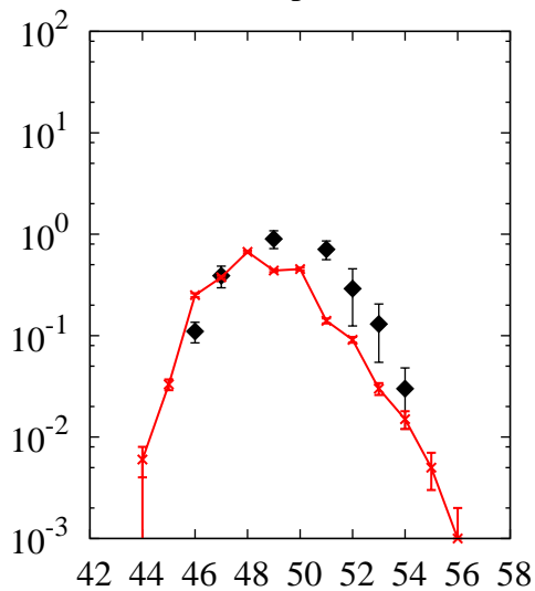
^{238}\text{U}(p,x)\text{Ti}
