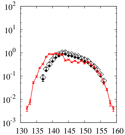
^{238}\text{U}(p,x)\text{Pm}
