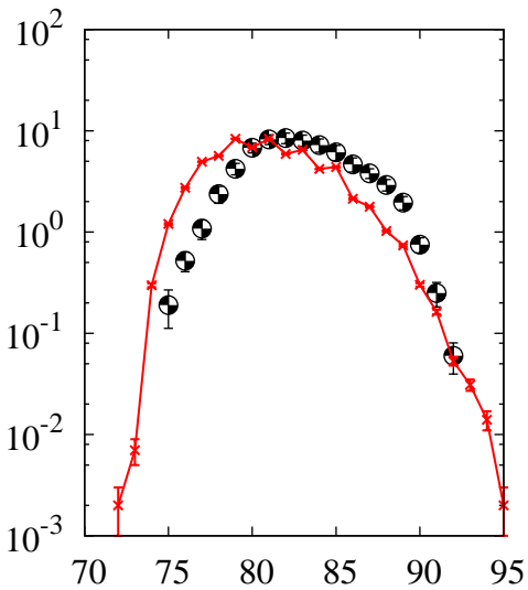
^{238}\text{U}(p,x)\text{Br}
