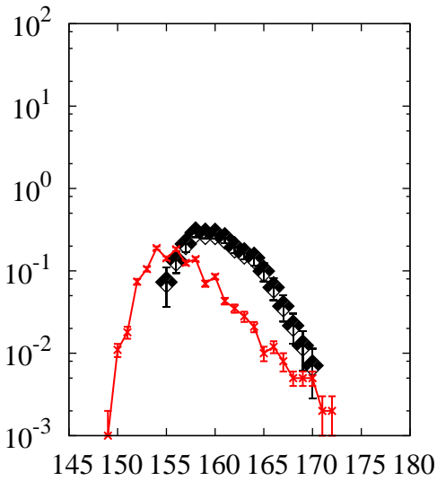
^{238}\text{U}(p,x)\text{Er}
