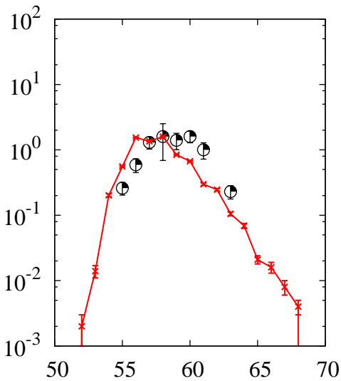
^{238}\text{U}(p,x)\text{Fe}
