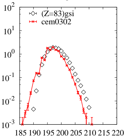
^{238}\text{U}(p,x)\text{Bi}
