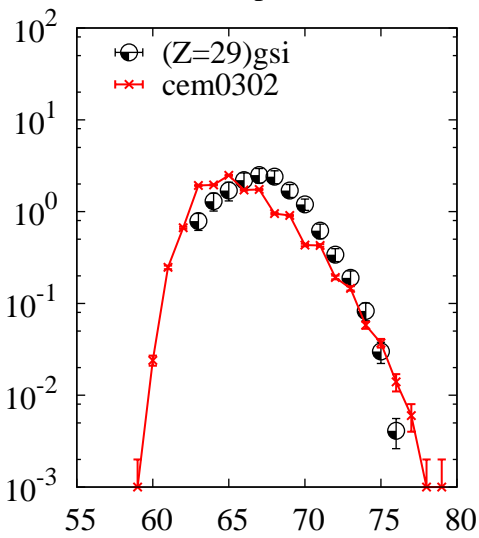
^{238}\text{U}(p,x)\text{Cu}
