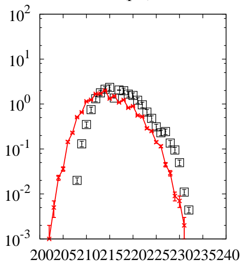
^{238}\text{U}(p,x)\text{Ra}
