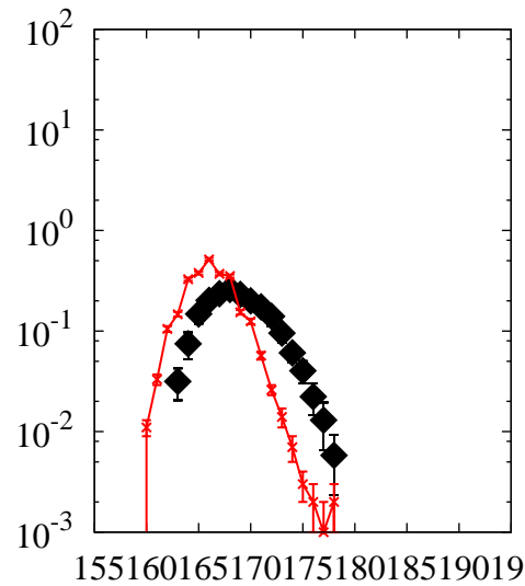
^{238}\text{U}(p,x)\text{Hf}
