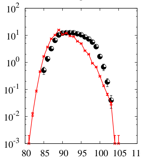
^{238}\text{U}(p,x)\text{Y}
