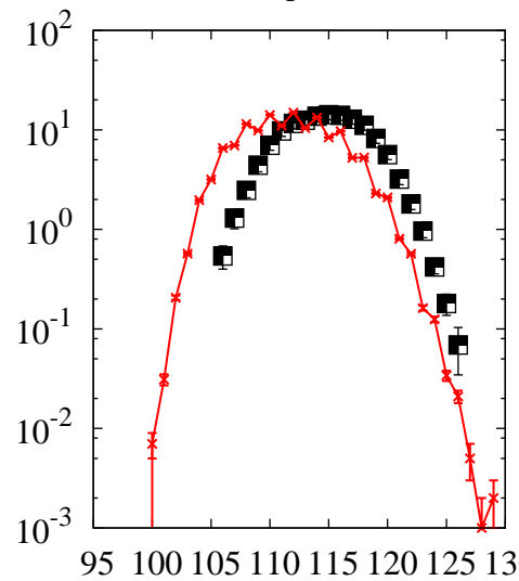
^{238}\text{U}(p,x)\text{Cd}
