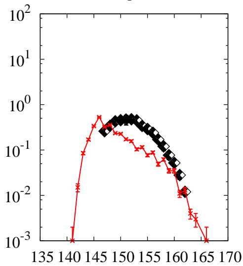
^{238}\text{U}(p,x)\text{Gd}
