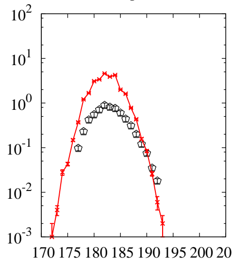
^{238}\text{U}(p,x)\text{Pt}
