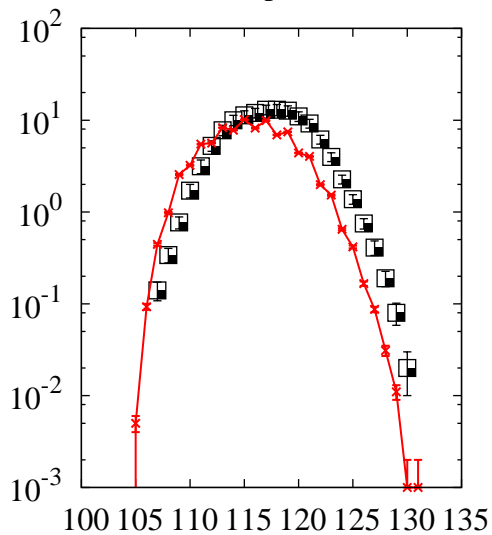
^{238}\text{U}(p,x)\text{In}
