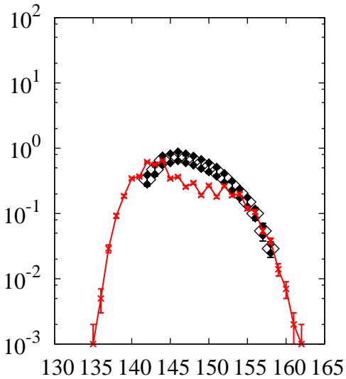
^{238}\text{U}(p,x)\text{Sm}
