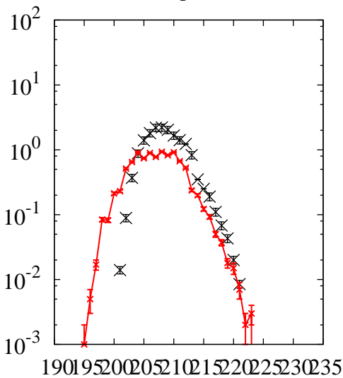
^{238}\text{U}(p,x)\text{Rn}
