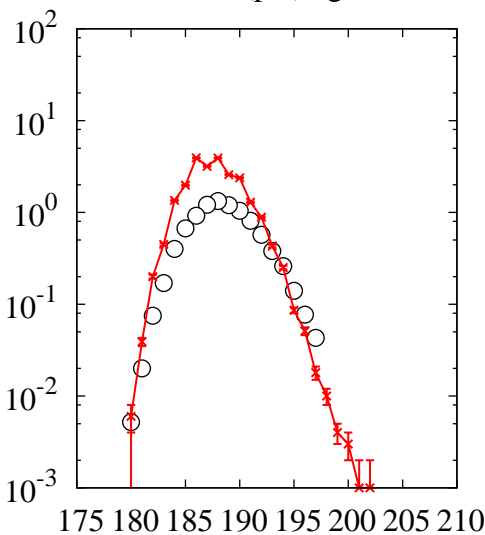
^{238}\text{U}(p,x)\text{Hg}
