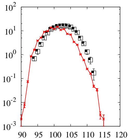
^{238}\text{U}(p,x)\text{Tc}
