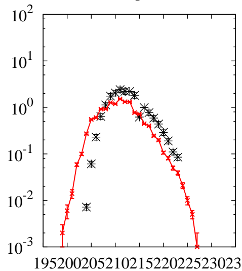
^{238}\text{U}(p,x)\text{Fr}
