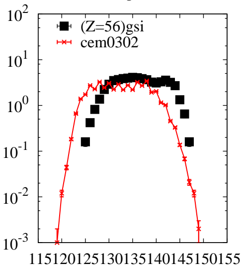
^{238}\text{U}(p,x)\text{Ba}
