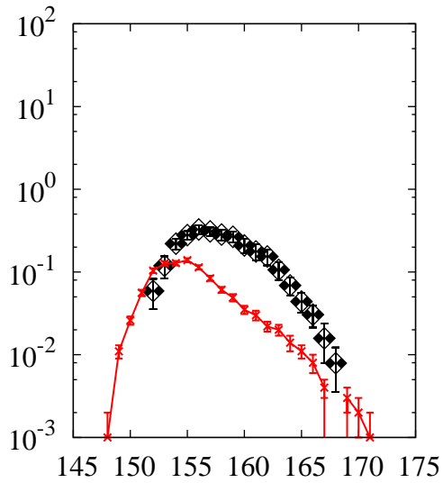
^{238}\text{U}(p,x)\text{Ho}
