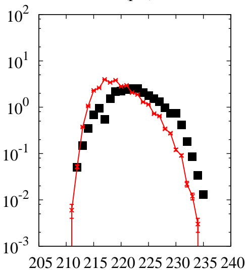
^{238}\text{U}(p,x)\text{Ac}
