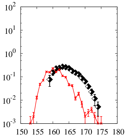
^{238}\text{U}(p,x)\text{Yb}
