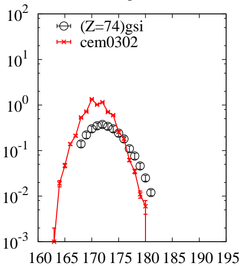
^{238}\text{U}(p,x)\text{W}
