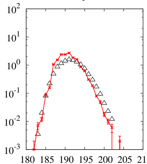
^{238}\text{U}(p,x)\text{Tl}
