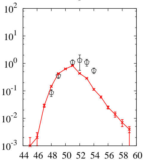
^{238}\text{U}(p,x)\text{V}
