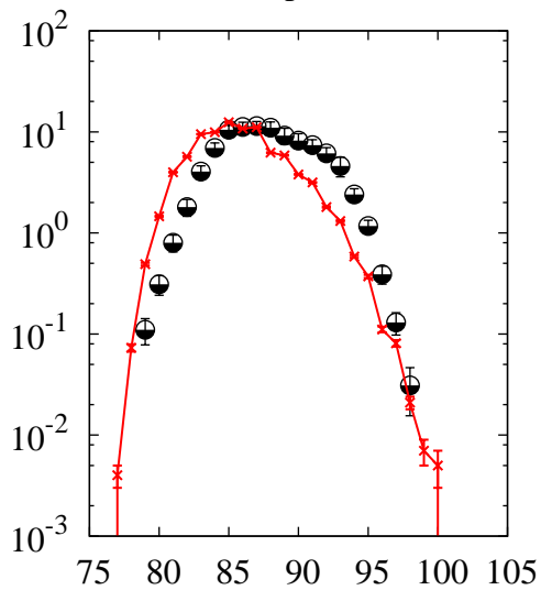
^{238}\text{U}(p,x)\text{Rb}
