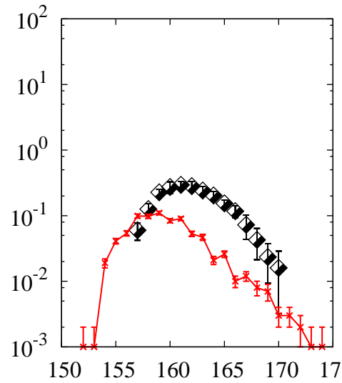
^{238}\text{U}(p,x)\text{Tm}
