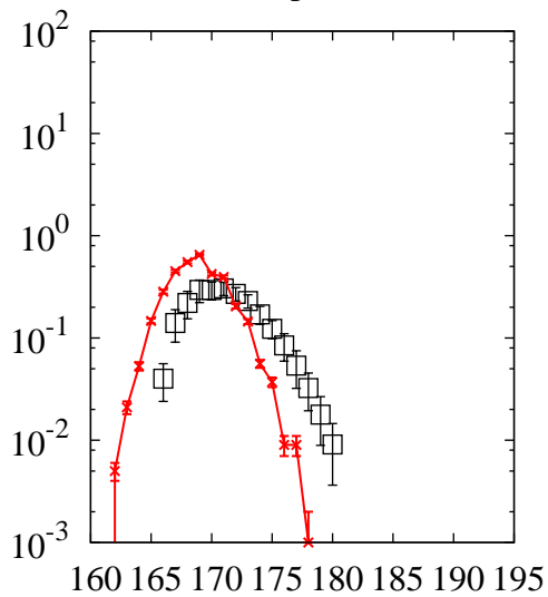
^{238}\text{U}(p,x)\text{Ta}
