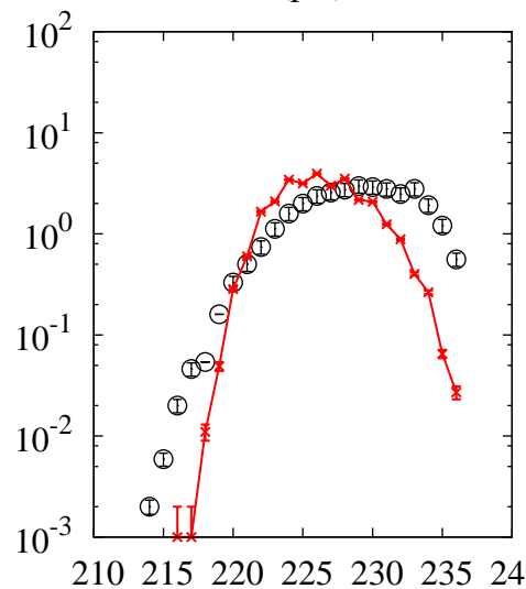
^{238}\text{U}(p,x)\text{Th}
