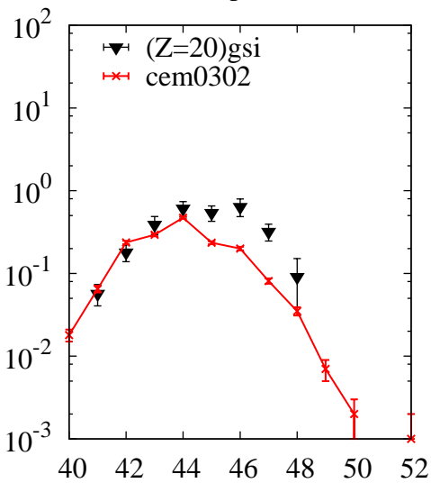
^{238}\text{U}(p,x)\text{Ca}
