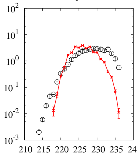
^{238}\text{U}(p,x)\text{Th}
