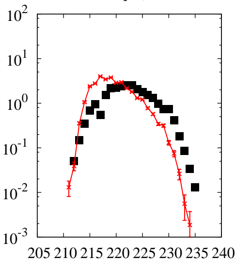
^{238}\text{U}(p,x)\text{Ac}
