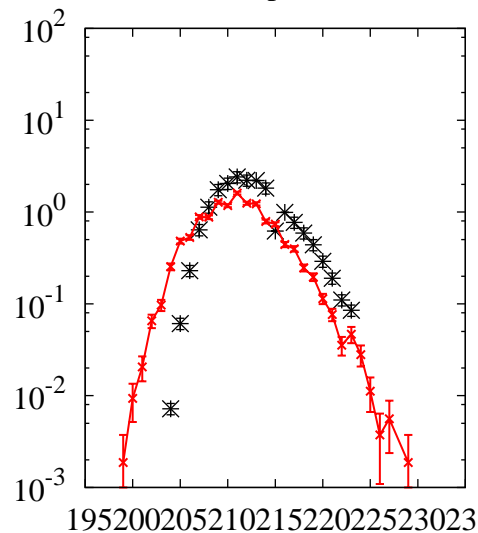
^{238}\text{U}(p,x)\text{Fr}
