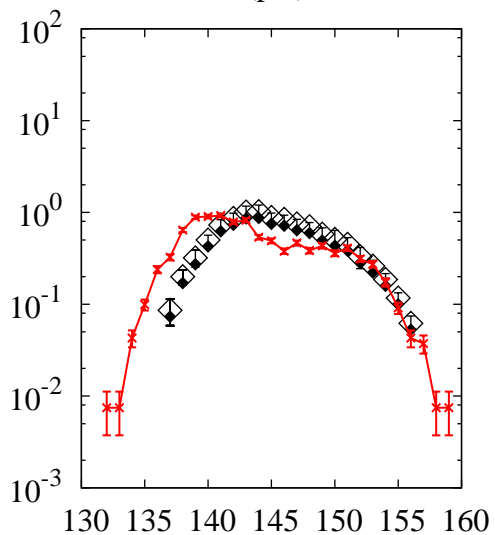
^{238}\text{U}(p,x)\text{Pm}
