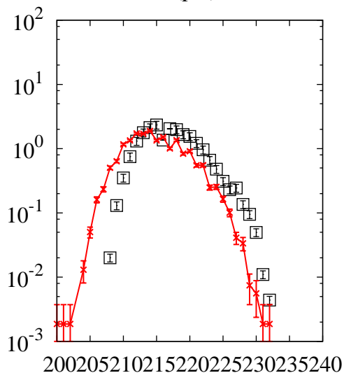
^{238}\text{U}(p,x)\text{Ra}
