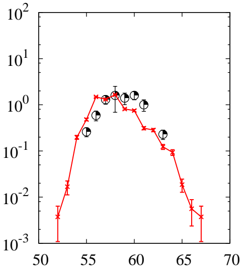
^{238}\text{U}(p,x)\text{Fe}
