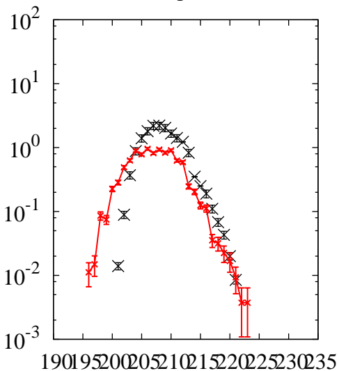
^{238}\text{U}(p,x)\text{Rn}
