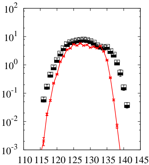
^{238}\text{U}(p,x)\text{I}
