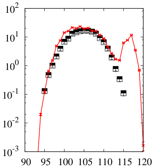
^{238}\text{U}(p,x)\text{Ru}
