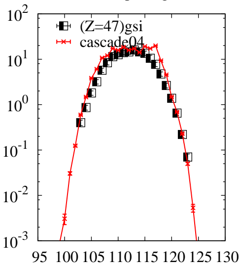
^{238}\text{U}(p,x)\text{Ag}
