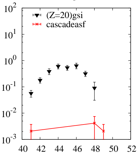
^{238}\text{U}(p,x)\text{Ca}
