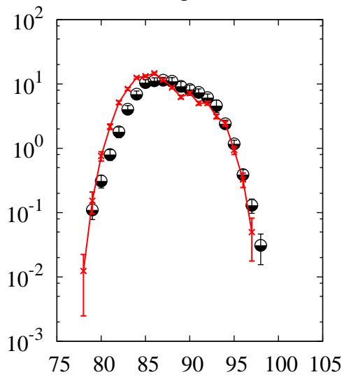
^{238}\text{U}(p,x)\text{Rb}
