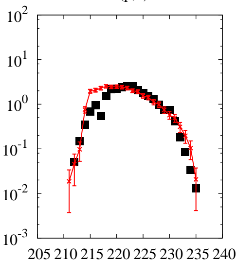
^{238}\text{U}(p,x)\text{Ac}
