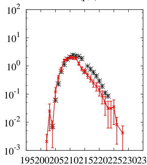
^{238}\text{U}(p,x)\text{Fr}
