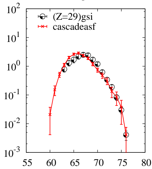
^{238}\text{U}(p,x)\text{Cu}
