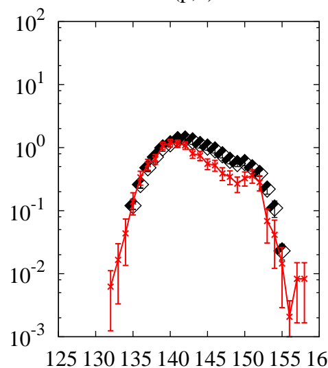
^{238}\text{U}(p,x)\text{Nd}
