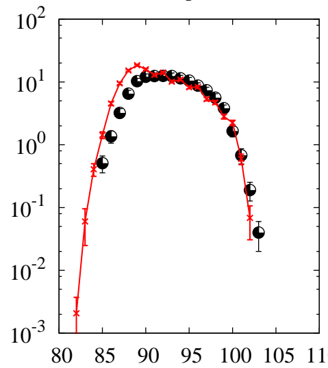
^{238}\text{U}(p,x)\text{Y}
