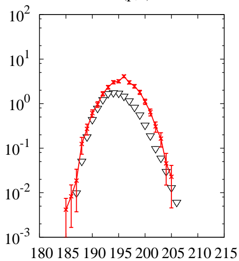
^{238}\text{U}(p,x)\text{Pb}
