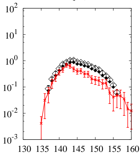
^{238}\text{U}(p,x)\text{Pm}
