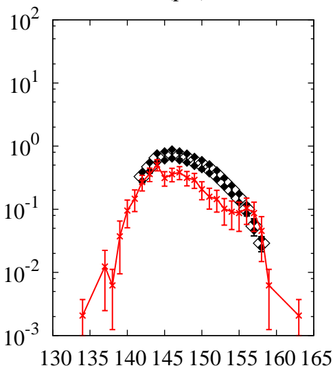
^{238}\text{U}(p,x)\text{Sm}
