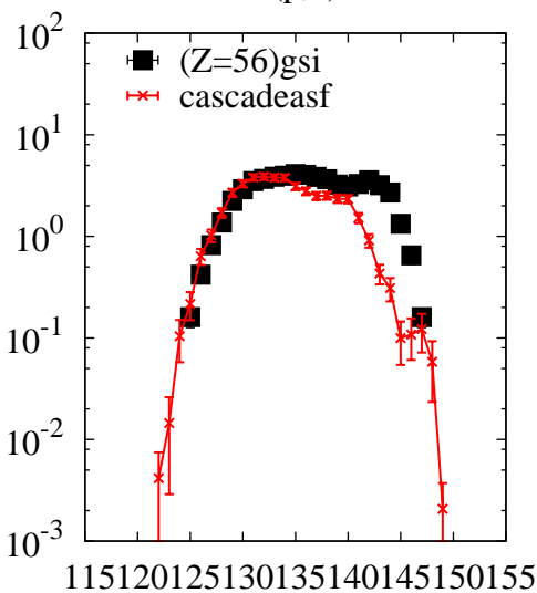
^{238}\text{U}(p,x)\text{Ba}
