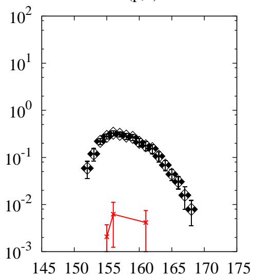
^{238}\text{U}(p,x)\text{Ho}
