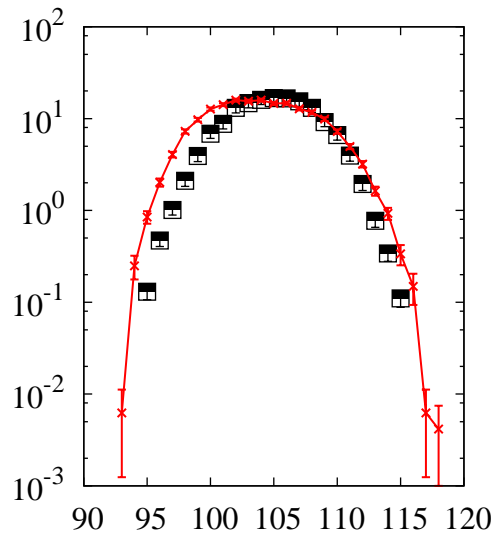
^{238}\text{U}(p,x)\text{Ru}
