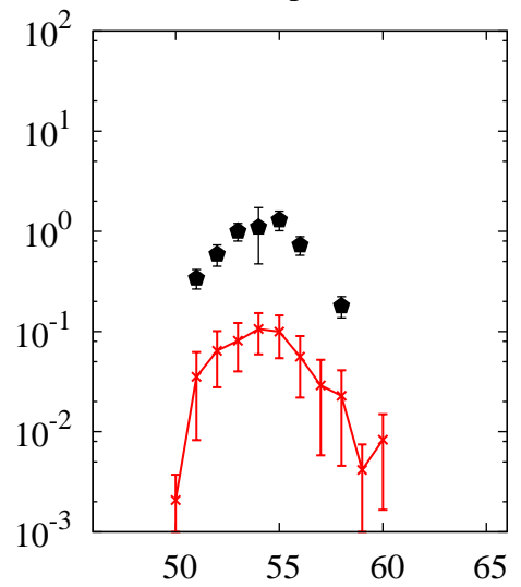
^{238}\text{U}(p,x)\text{Cr}
