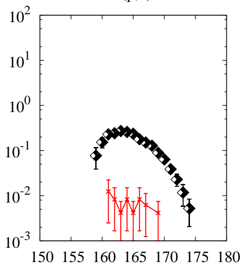
^{238}\text{U}(p,x)\text{Yb}
