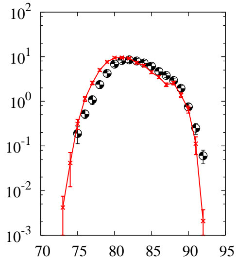
^{238}\text{U}(p,x)\text{Br}
