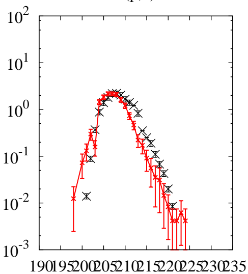
^{238}\text{U}(p,x)\text{Rn}
