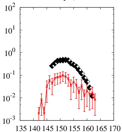
^{238}\text{U}(p,x)\text{Gd}
