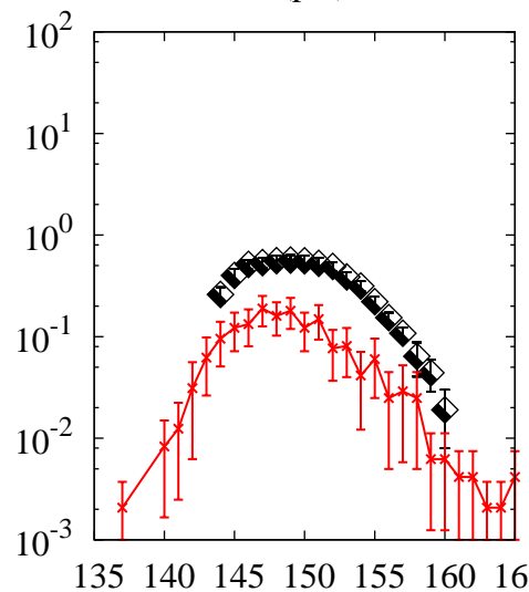
^{238}\text{U}(p,x)\text{Eu}
