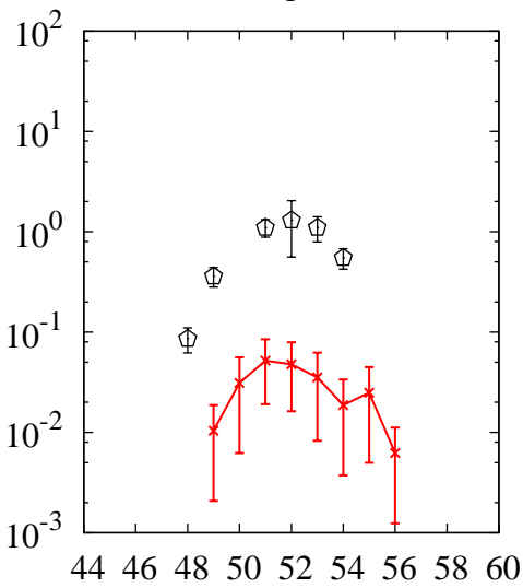
^{238}\text{U}(p,x)\text{V}
