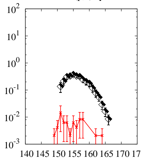
^{238}\text{U}(p,x)\text{Dy}
