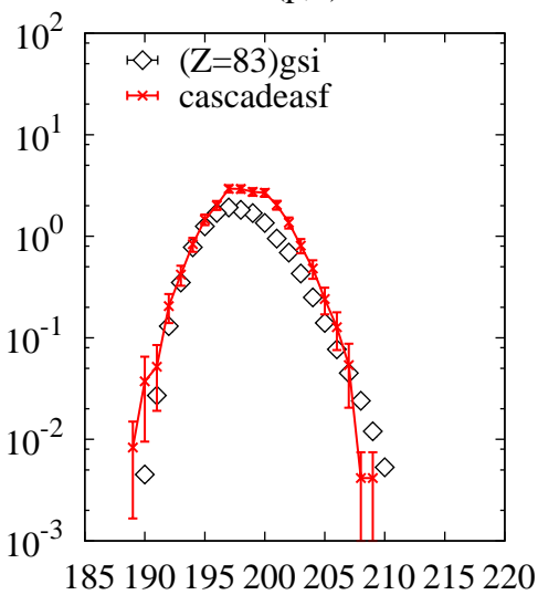
^{238}\text{U}(p,x)\text{Bi}
