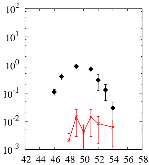
^{238}\text{U}(p,x)\text{Ti}
