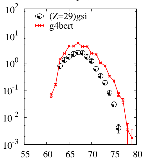
^{238}\text{U}(p,x)\text{Cu}
