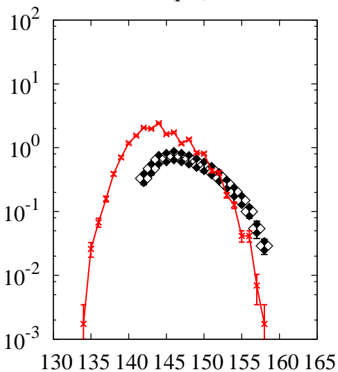
^{238}\text{U}(p,x)\text{Sm}
