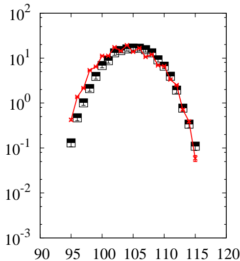
^{238}\text{U}(p,x)\text{Ru}
