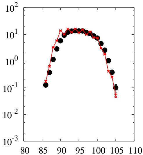
^{238}\text{U}(p,x)\text{Zr}
