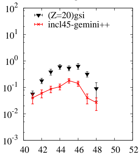
^{238}\text{U}(p,x)\text{Ca}
