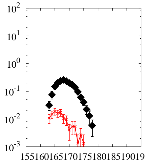
^{238}\text{U}(p,x)\text{Hf}
