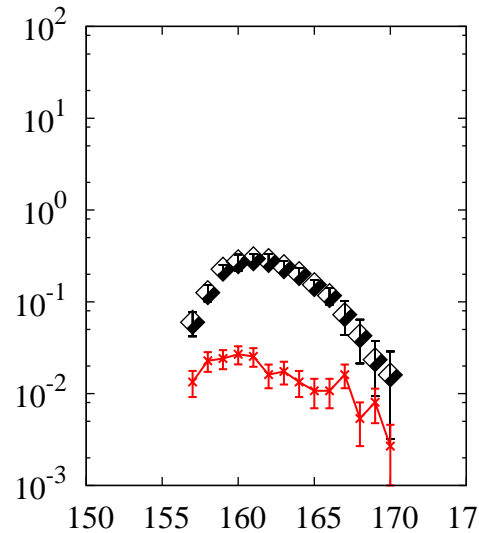
^{238}\text{U}(p,x)\text{Tm}
