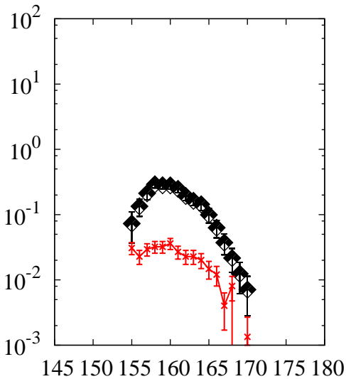
^{238}\text{U}(p,x)\text{Er}
