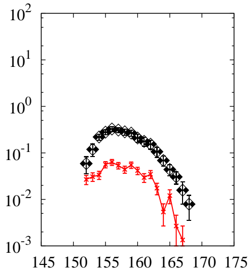
^{238}\text{U}(p,x)\text{Ho}
