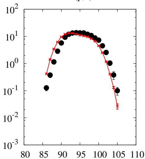
^{238}\text{U}(p,x)\text{Zr}
