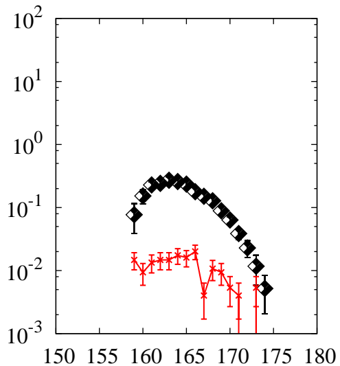
^{238}\text{U}(p,x)\text{Yb}
