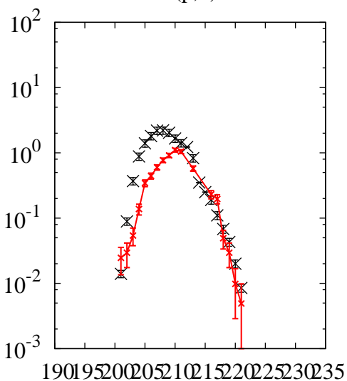
^{238}\text{U}(p,x)\text{Rn}
