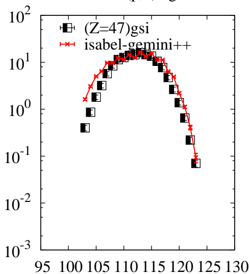
^{238}\text{U}(p,x)\text{Ag}
