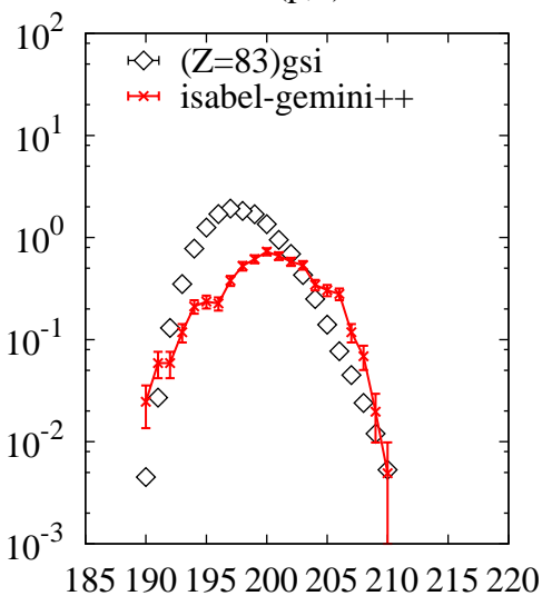
^{238}\text{U}(p,x)\text{Bi}
