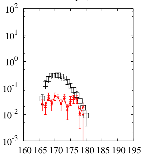
^{238}\text{U}(p,x)\text{Ta}
