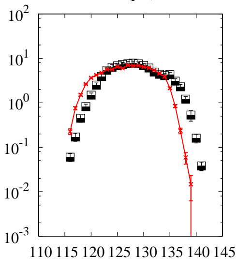
^{238}\text{U}(p,x)\text{I}
