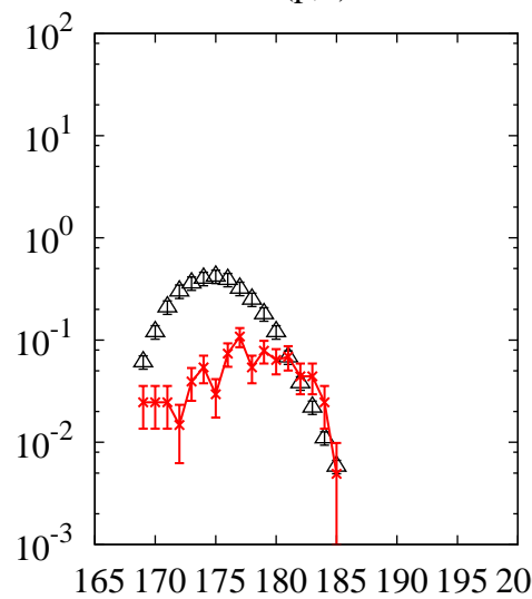
^{238}\text{U}(p,x)\text{Re}
