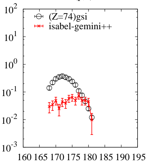
^{238}\text{U}(p,x)\text{W}
