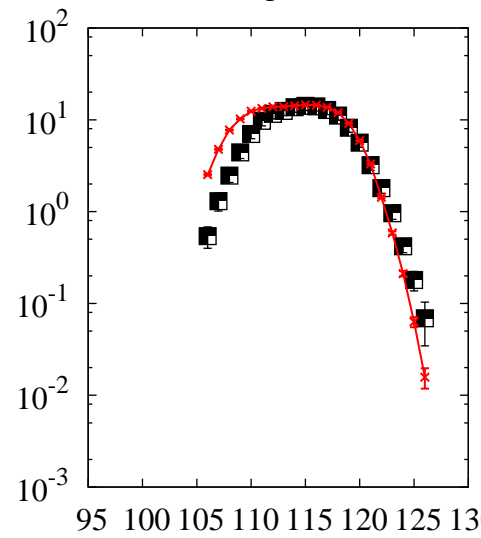
^{238}\text{U}(p,x)\text{Cd}
