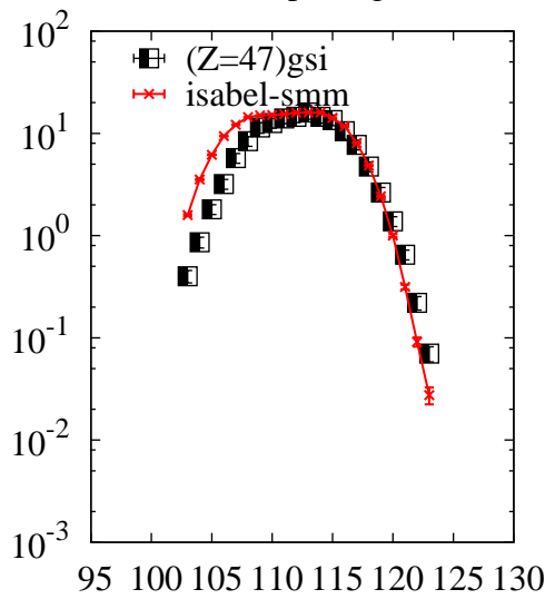
^{238}\text{U}(p,x)\text{Ag}
