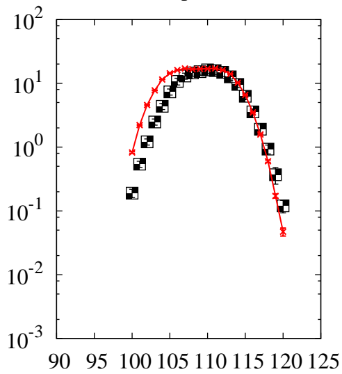
^{238}\text{U}(p,x)\text{Pd}
