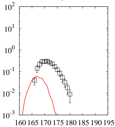
^{238}\text{U}(p,x)\text{Ta}
