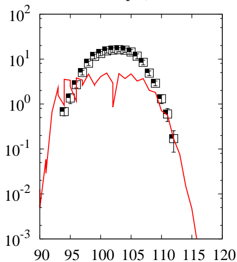
^{238}\text{U}(p,x)\text{Tc}
