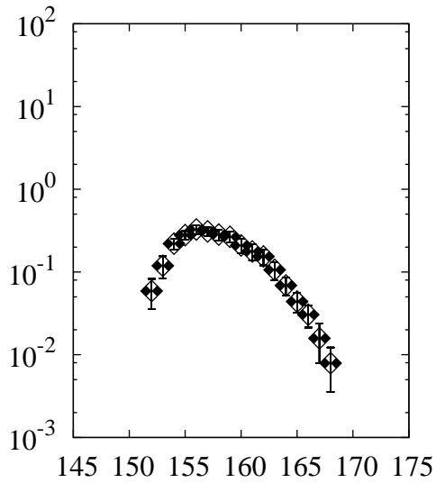
^{238}\text{U}(p,x)\text{Ho}
