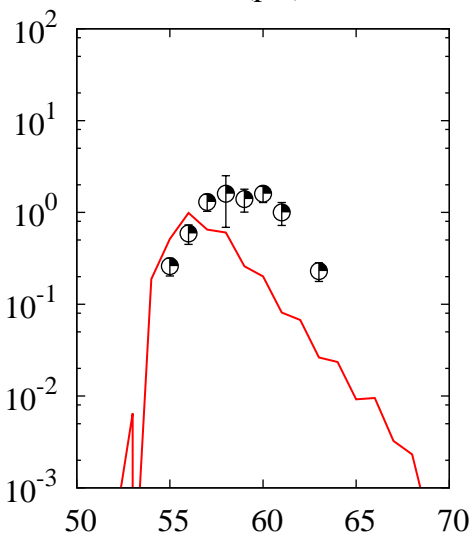
^{238}\text{U}(p,x)\text{Fe}
