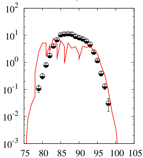
^{238}\text{U}(p,x)\text{Rb}
