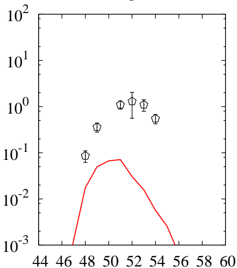
^{238}\text{U}(p,x)\text{V}
