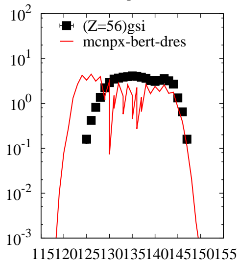
^{238}\text{U}(p,x)\text{Ba}
