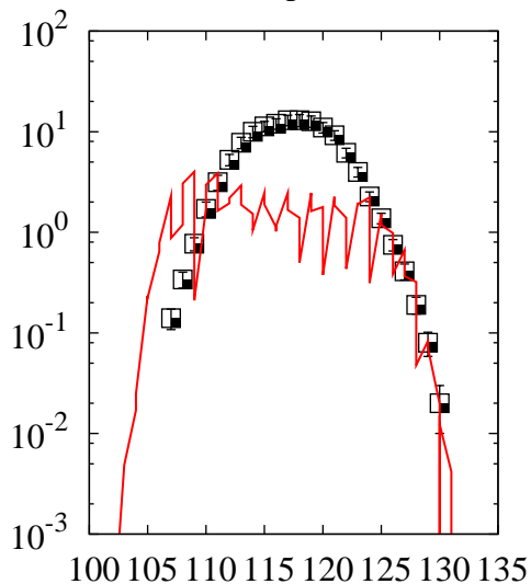
^{238}\text{U}(p,x)\text{In}
