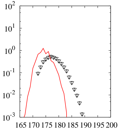
^{238}\text{U}(p,x)\text{Os}
