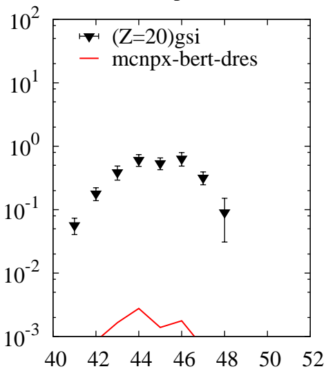
^{238}\text{U}(p,x)\text{Ca}
