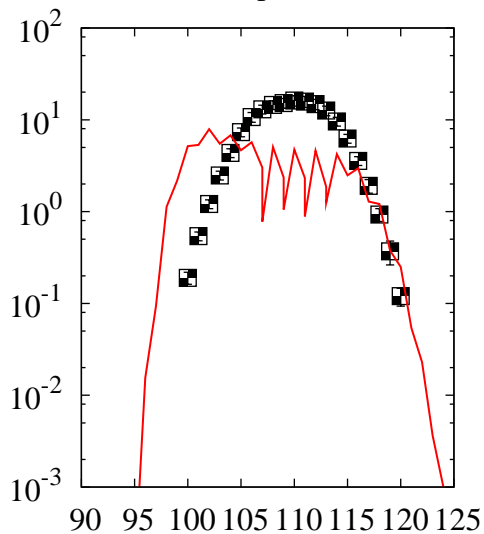
^{238}\text{U}(p,x)\text{Pd}
