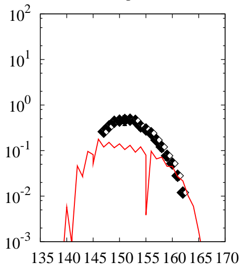
^{238}\text{U}(p,x)\text{Gd}
