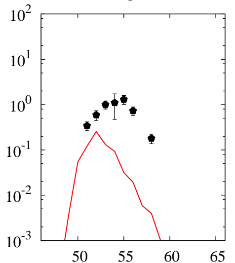
^{238}\text{U}(p,x)\text{Cr}
