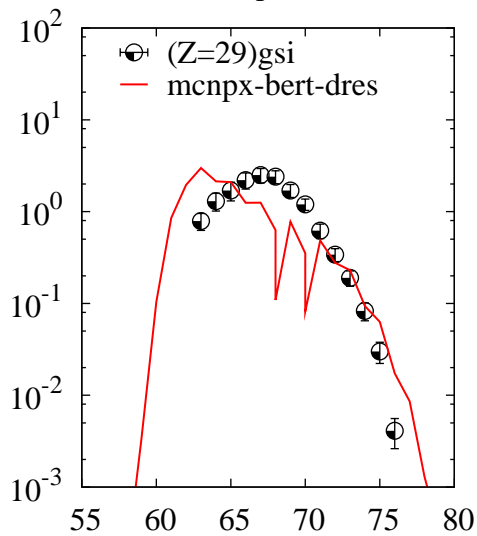
^{238}\text{U}(p,x)\text{Cu}
