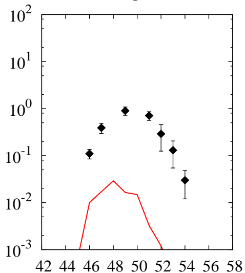
^{238}\text{U}(p,x)\text{Ti}
