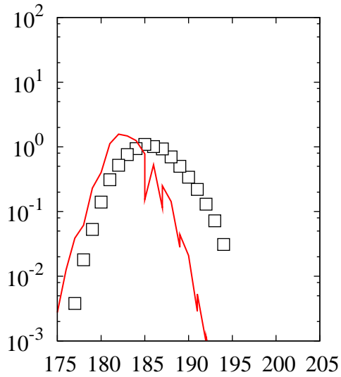
^{238}\text{U}(p,x)\text{Au}
