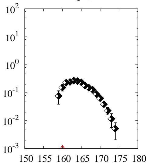
^{238}\text{U}(p,x)\text{Yb}
