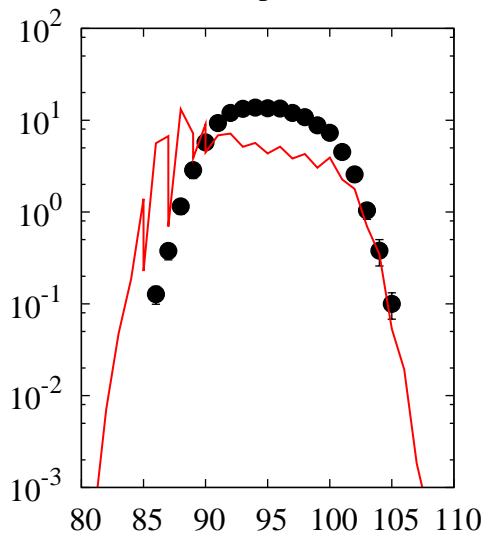
^{238}\text{U}(p,x)\text{Zr}
