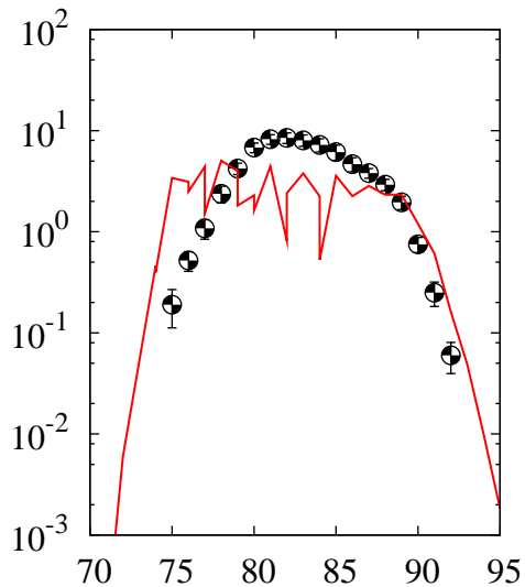
^{238}\text{U}(p,x)\text{Br}
