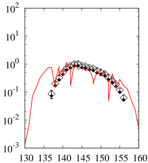
^{238}\text{U}(p,x)\text{Pm}
