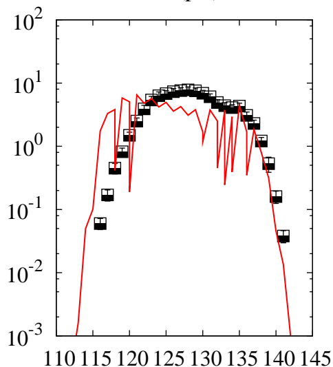
^{238}\text{U}(p,x)\text{I}
