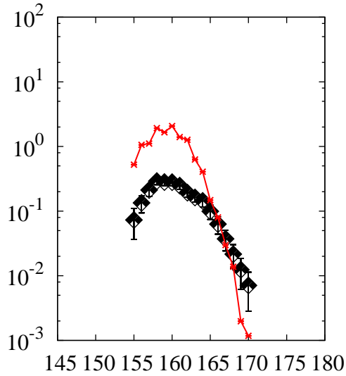
^{238}\text{U}(p,x)\text{Er}
