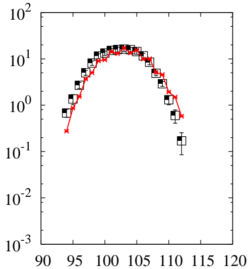
^{238}\text{U}(p,x)\text{Tc}
