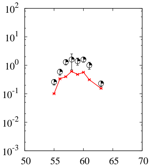
^{238}\text{U}(p,x)\text{Fe}
