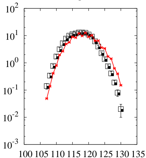
^{238}\text{U}(p,x)\text{In}
