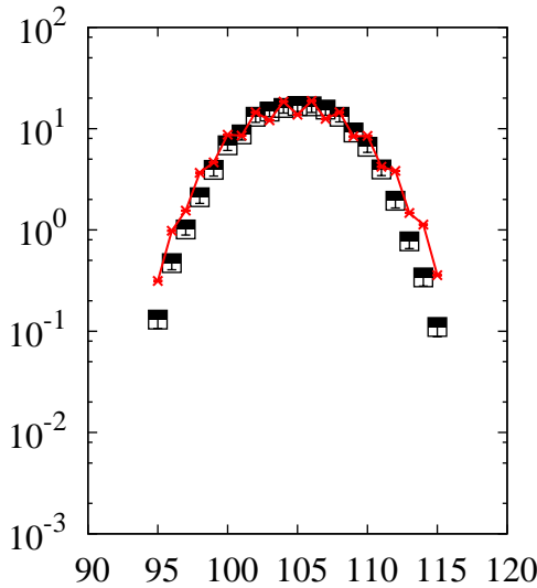
^{238}\text{U}(p,x)\text{Ru}
