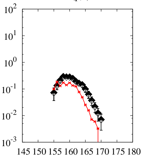
^{238}\text{U}(p,x)\text{Er}
