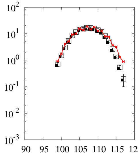
^{238}\text{U}(p,x)\text{Rh}
