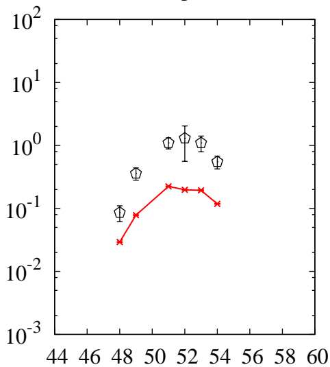
^{238}\text{U}(p,x)\text{V}
