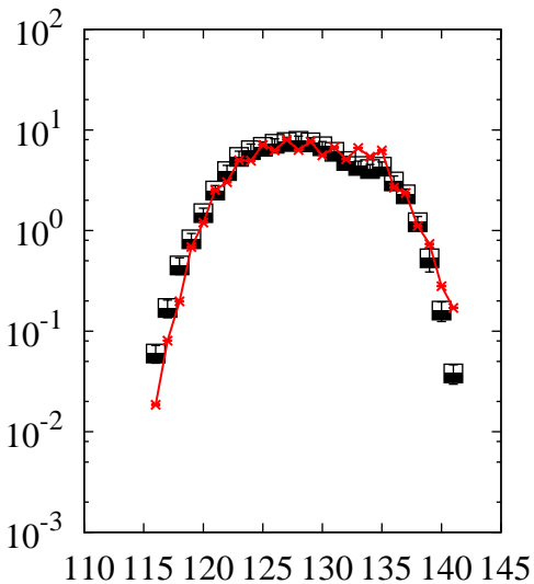
^{238}\text{U}(p,x)\text{I}
