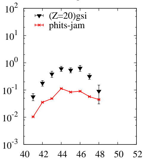
^{238}\text{U}(p,x)\text{Ca}
