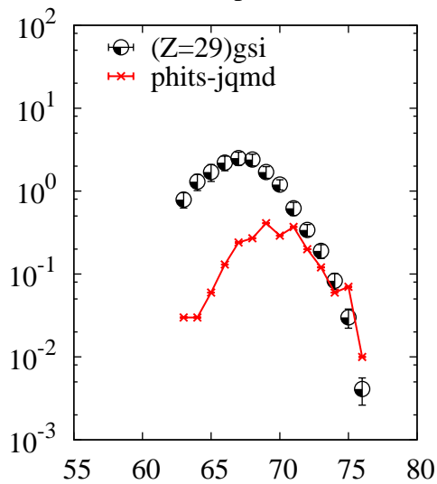
^{238}\text{U}(p,x)\text{Cu}
