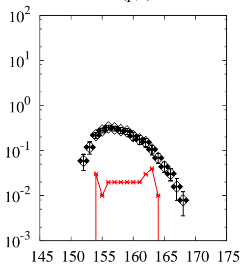
^{238}\text{U}(p,x)\text{Ho}
