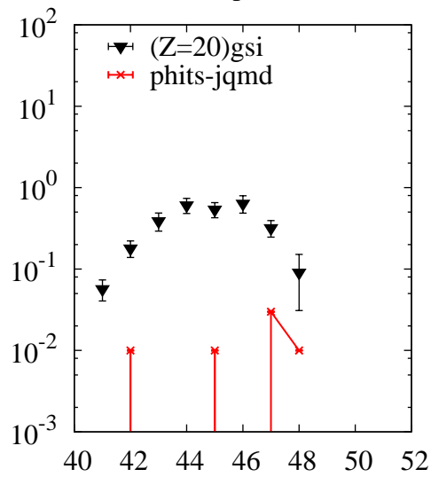
^{238}\text{U}(p,x)\text{Ca}
