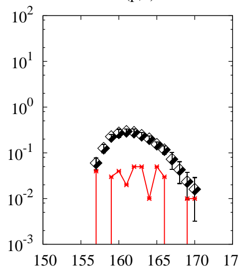
^{238}\text{U}(p,x)\text{Tm}
