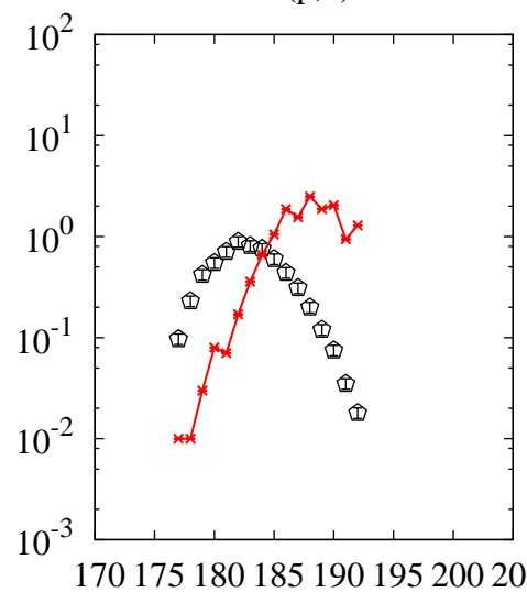
^{238}\text{U}(p,x)\text{Pt}
