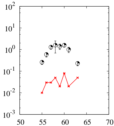
^{238}\text{U}(p,x)\text{Fe}
