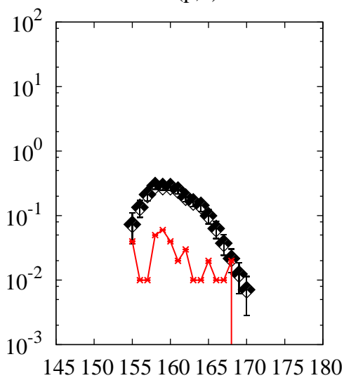
^{238}\text{U}(p,x)\text{Er}
