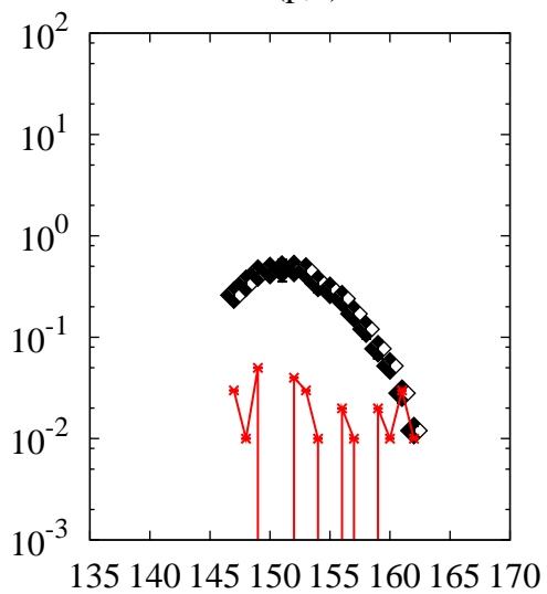
^{238}\text{U}(p,x)\text{Gd}
