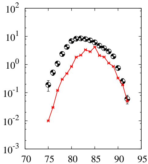
^{238}\text{U}(p,x)\text{Br}
