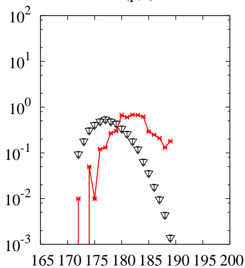
^{238}\text{U}(p,x)\text{Os}
