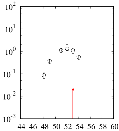
^{238}\text{U}(p,x)\text{V}
