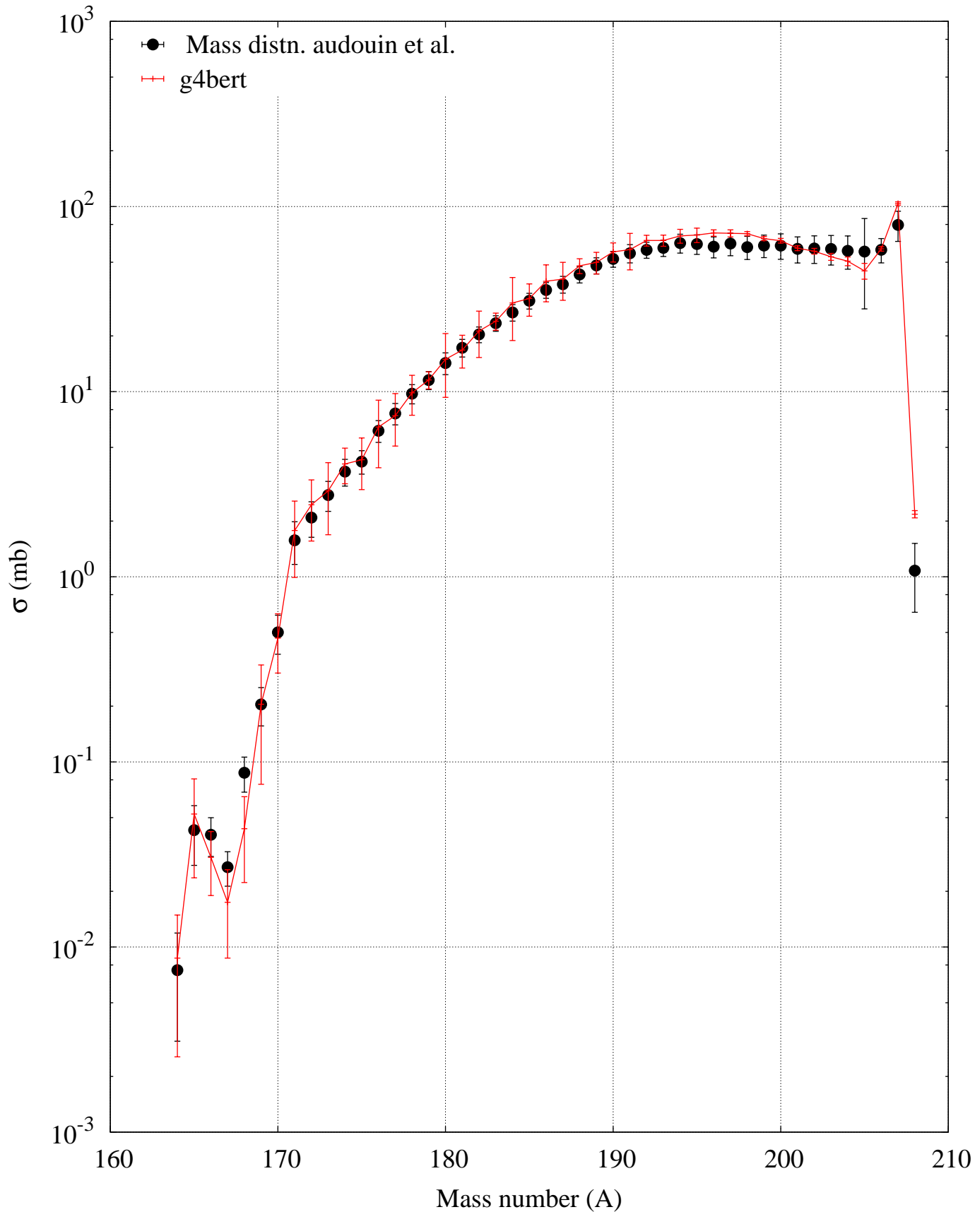
p (500 MeV) + Pb208 -- Residue mass production
