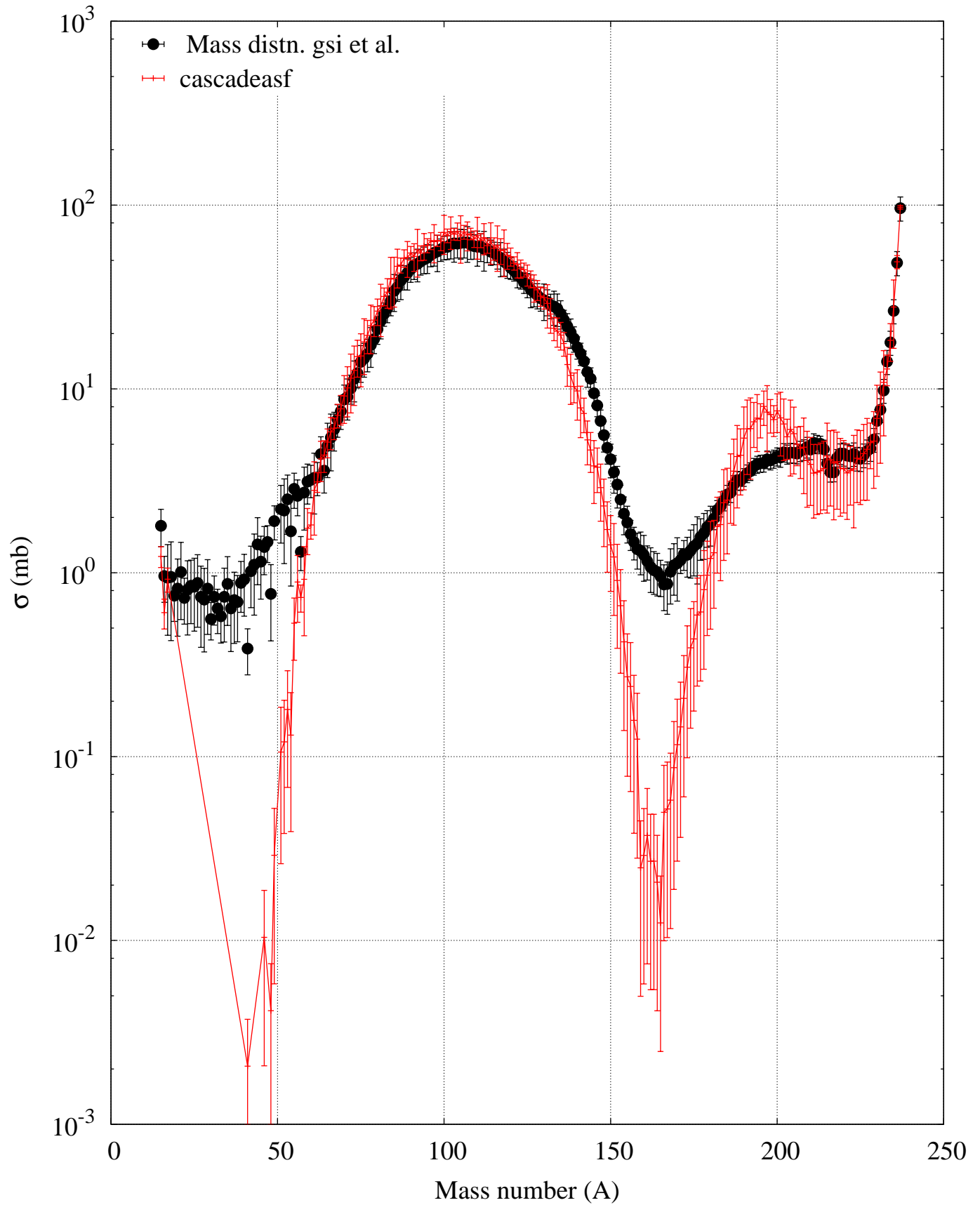
p (1000 MeV) + U238 -- Residue mass production
