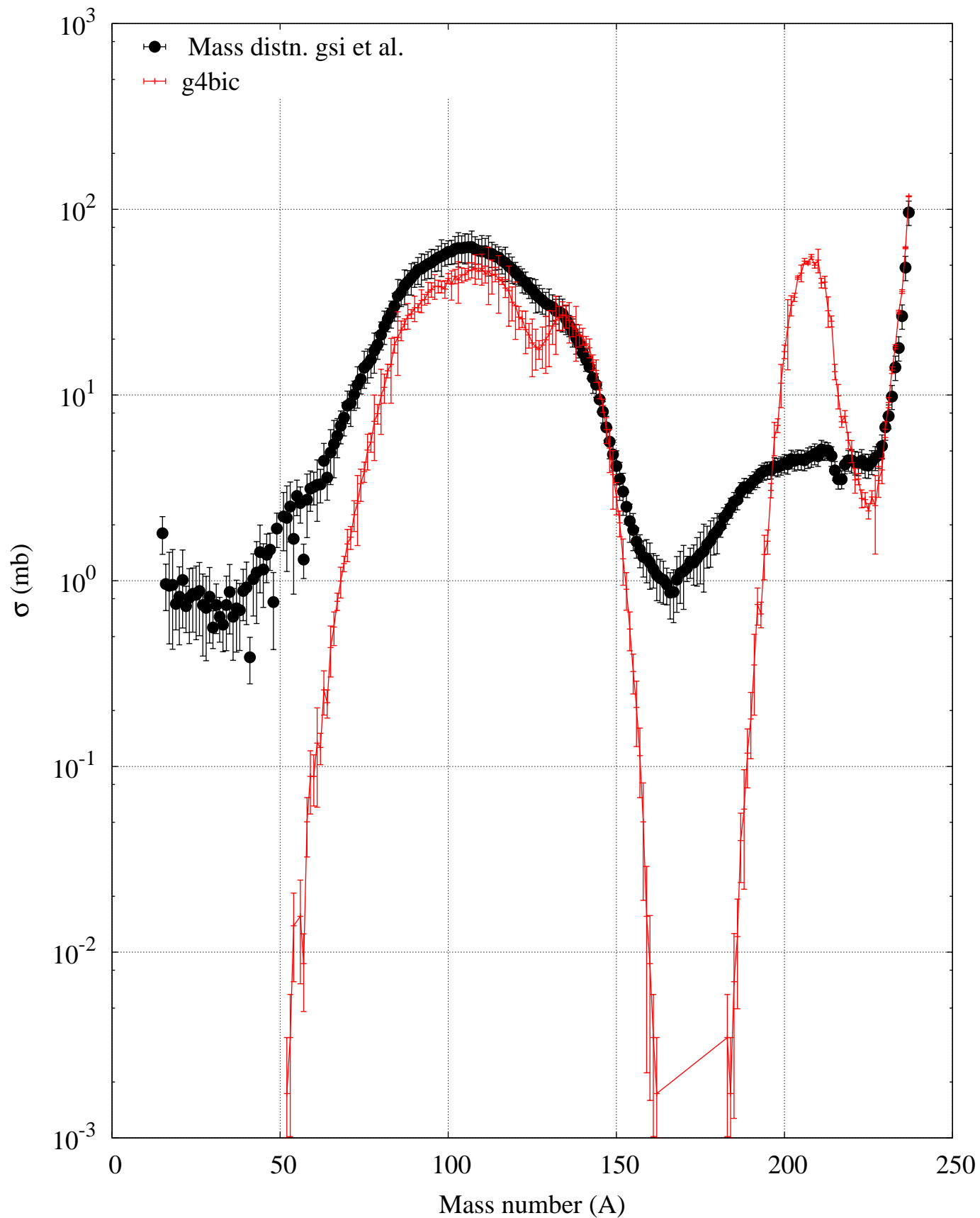
p (1000 MeV) + U238 -- Residue mass production
