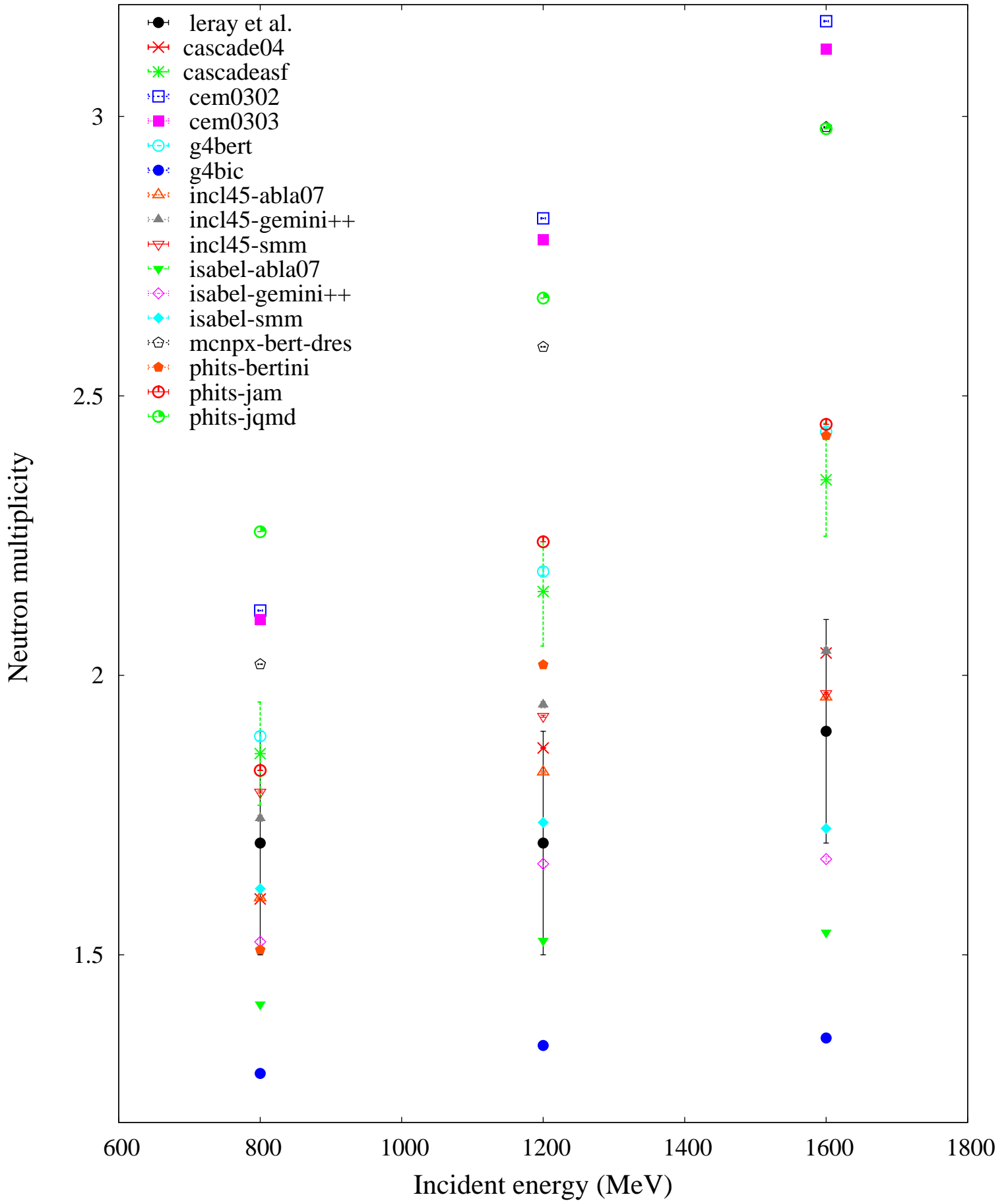
p + Fe -- (2-20 MeV) Avg. neutron multiplicities
