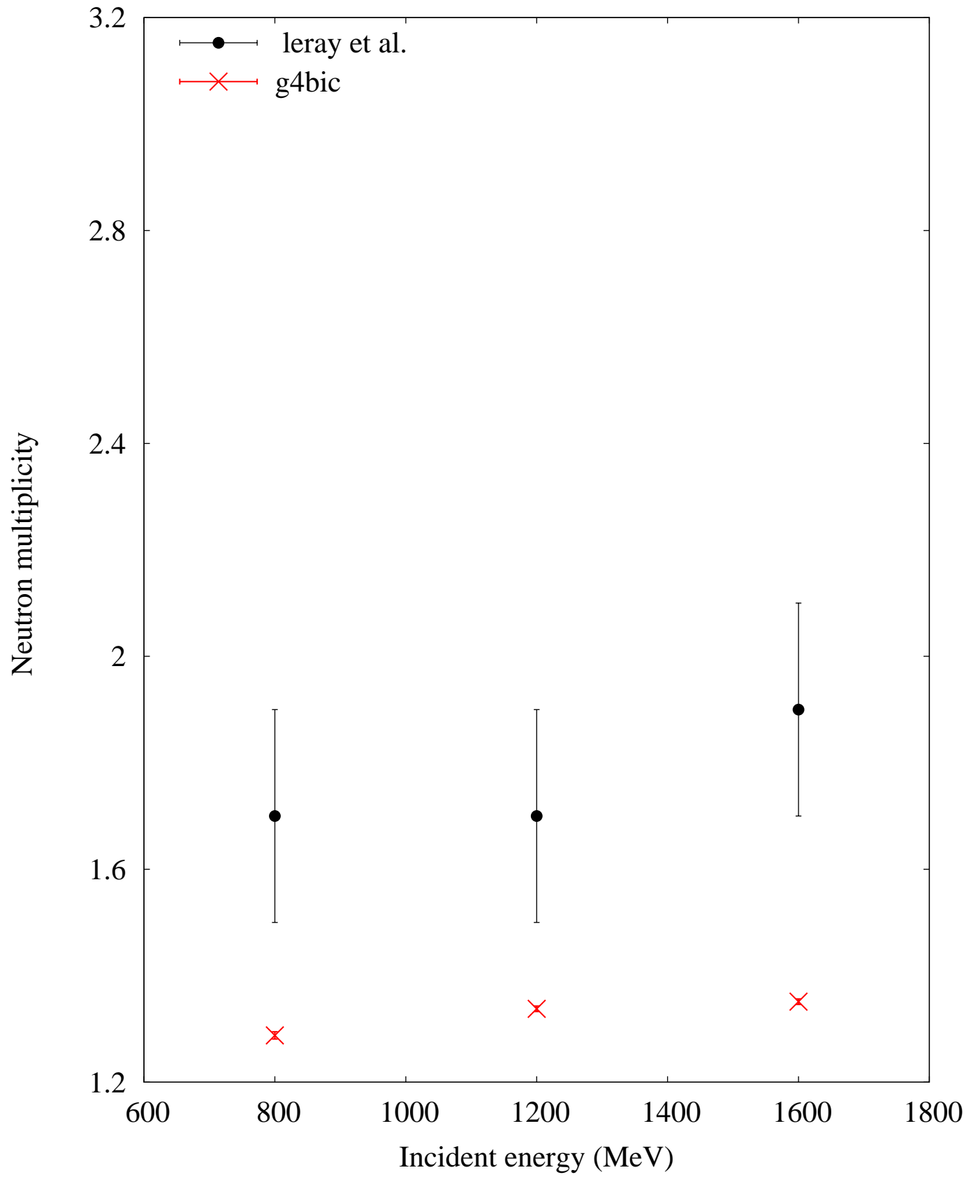
p + Fe -- (2-20 MeV) Avg. neutron multiplicities
