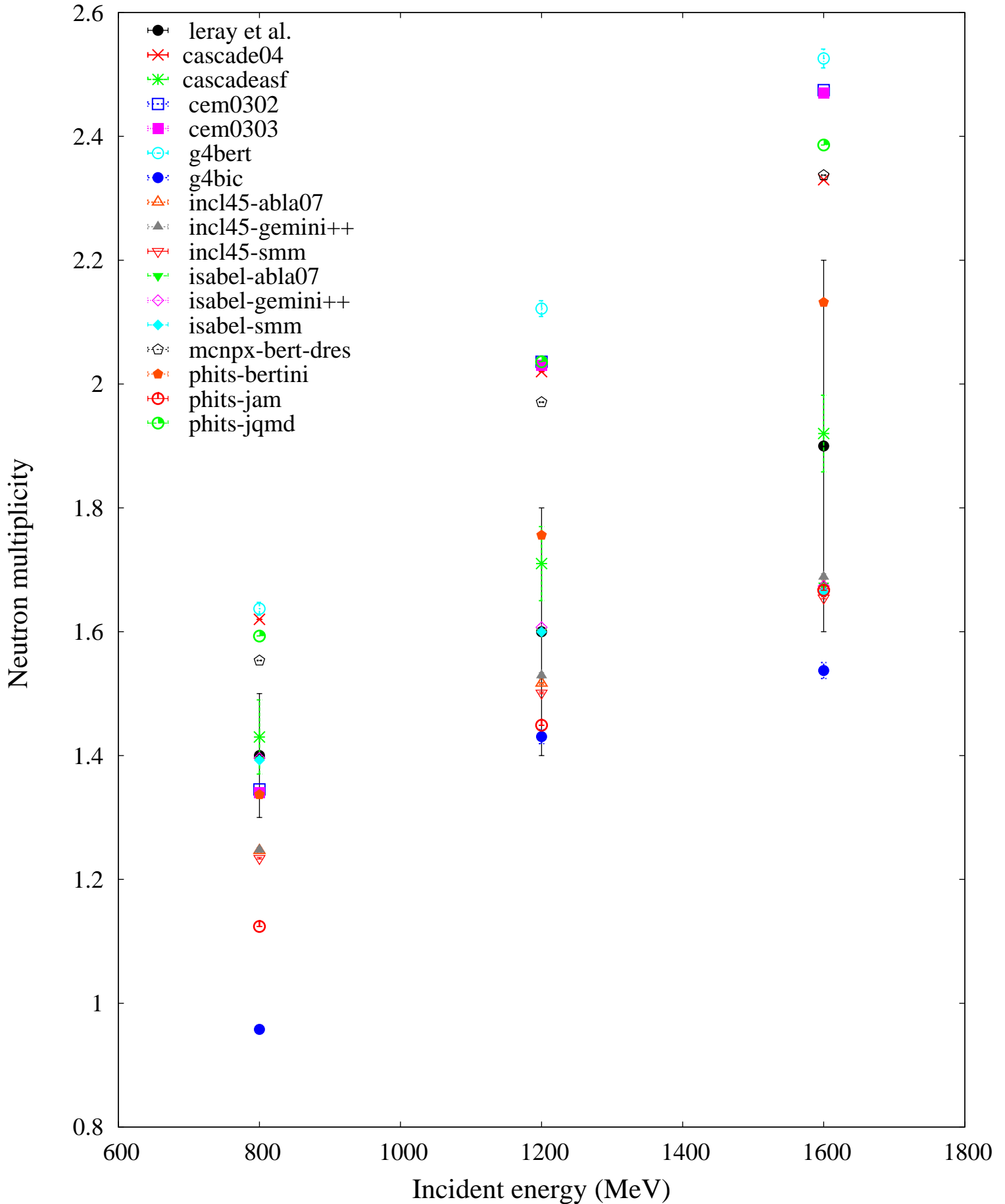
p + Fe -- (20+ MeV) Avg. neutron multiplicities
