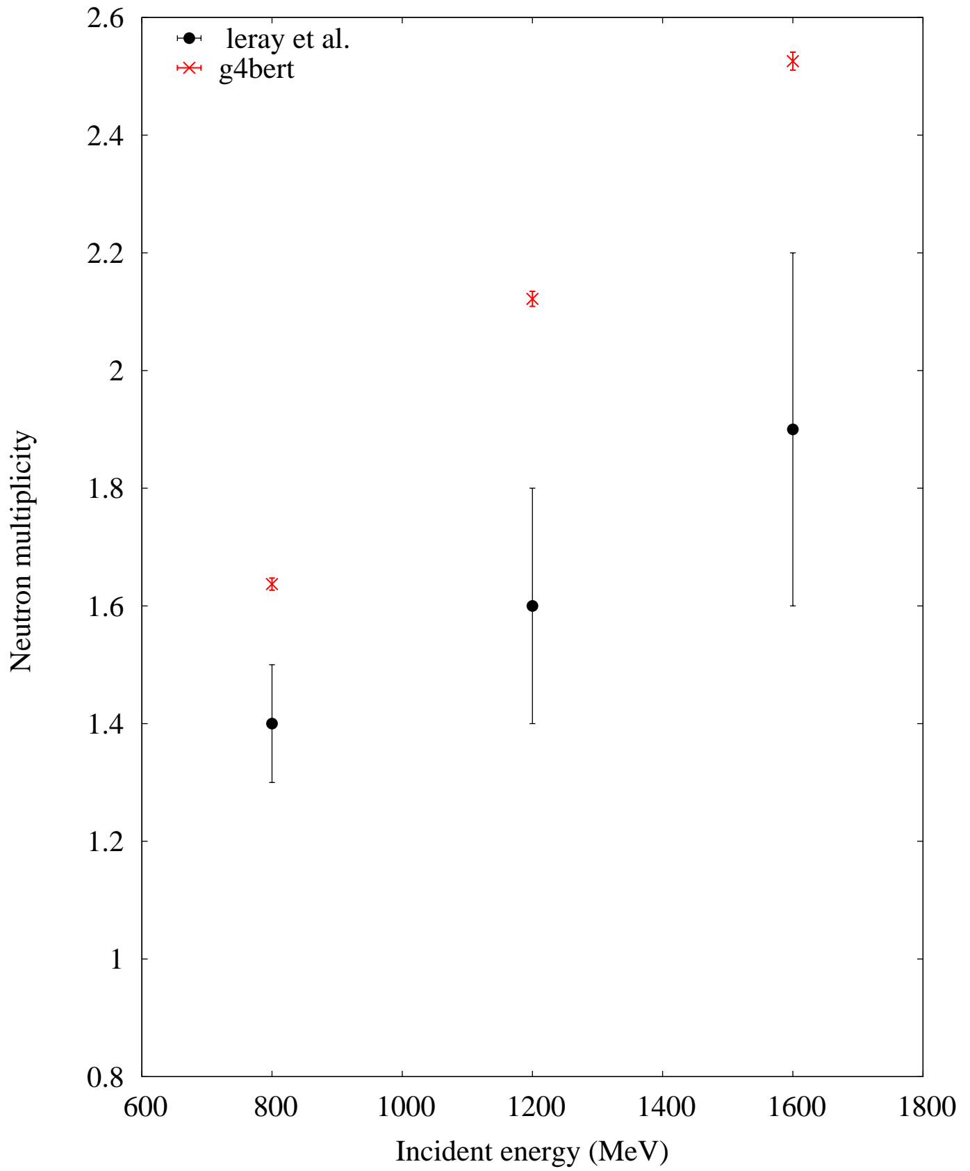
p + Fe -- (20+ MeV) Avg. neutron multiplicities
