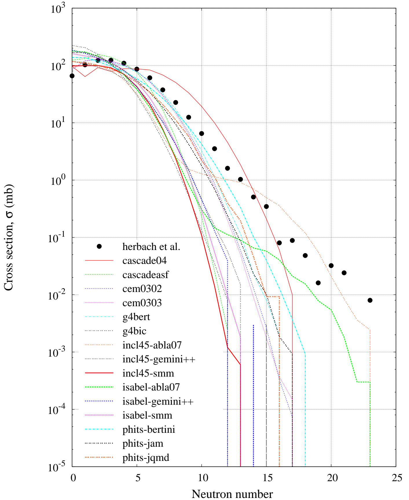
p (1200 MeV) + Fe -- Multiplicity distribution
