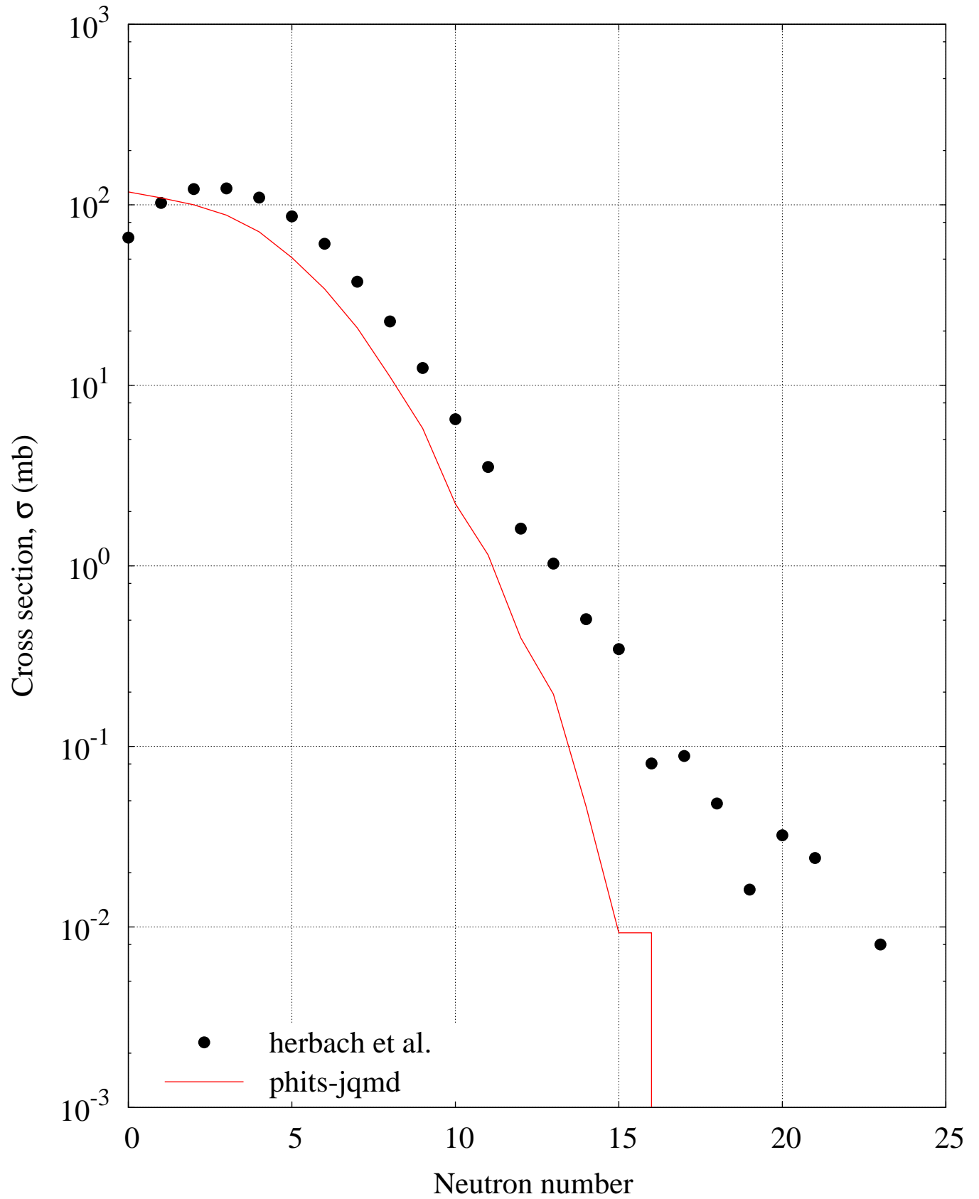
p (1200 MeV) + Fe --Multiplicity distribution
