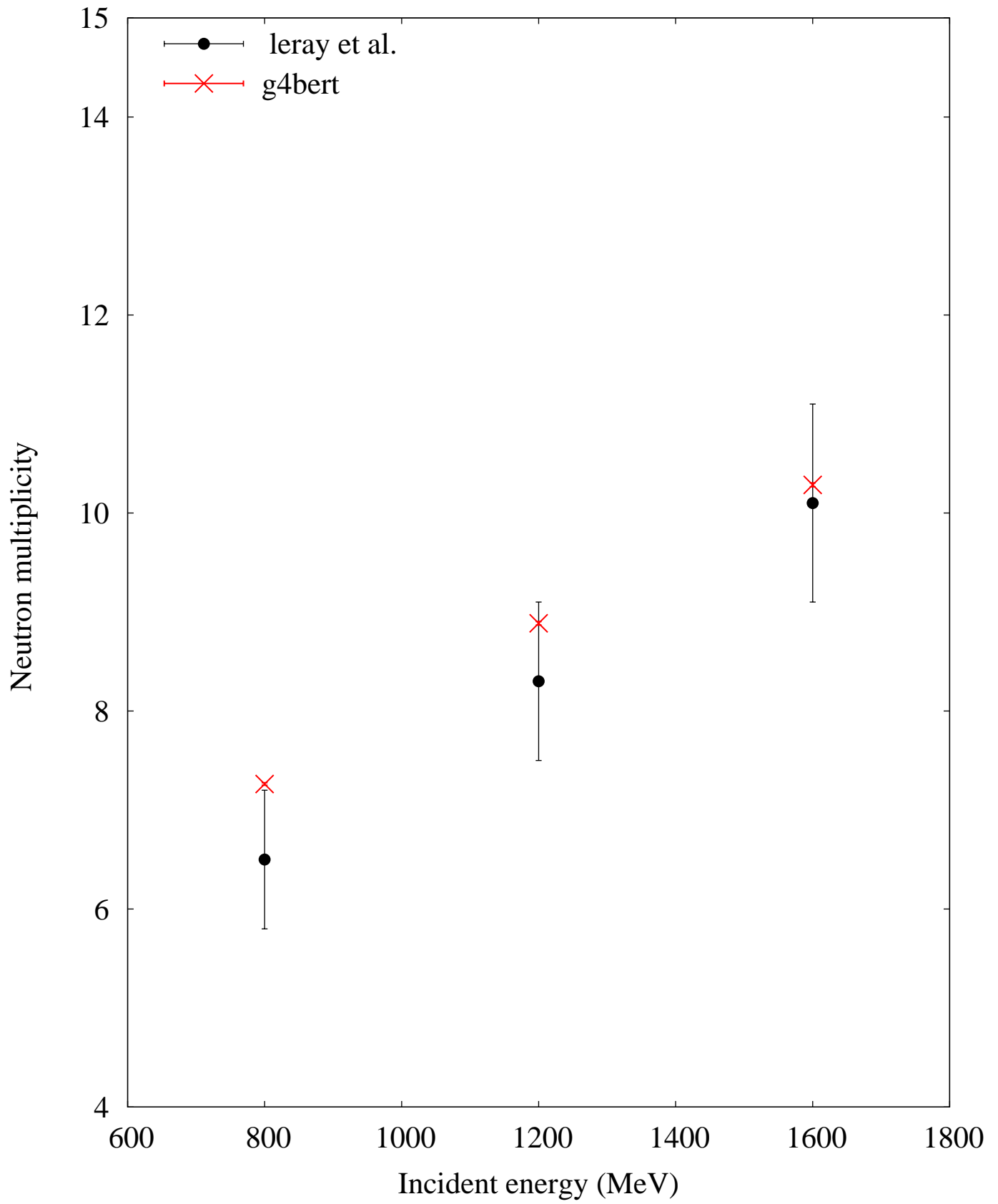
p + Pb -- (2-20 MeV) Avg. neutron multiplicities
