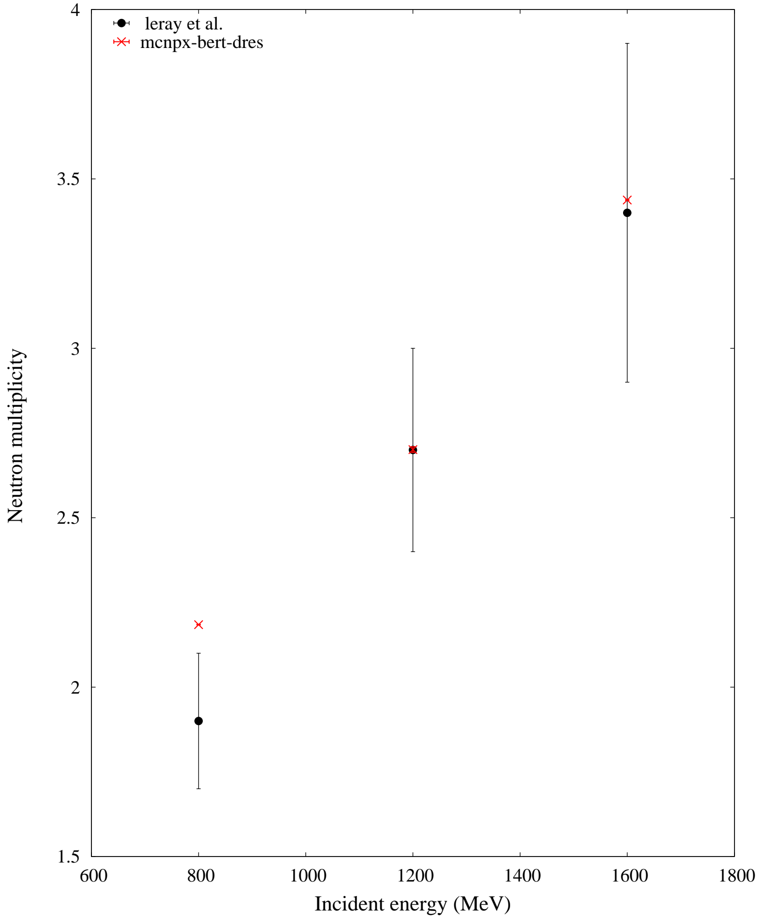
p + Pb -- (20+ MeV) Avg. neutron multiplicities
