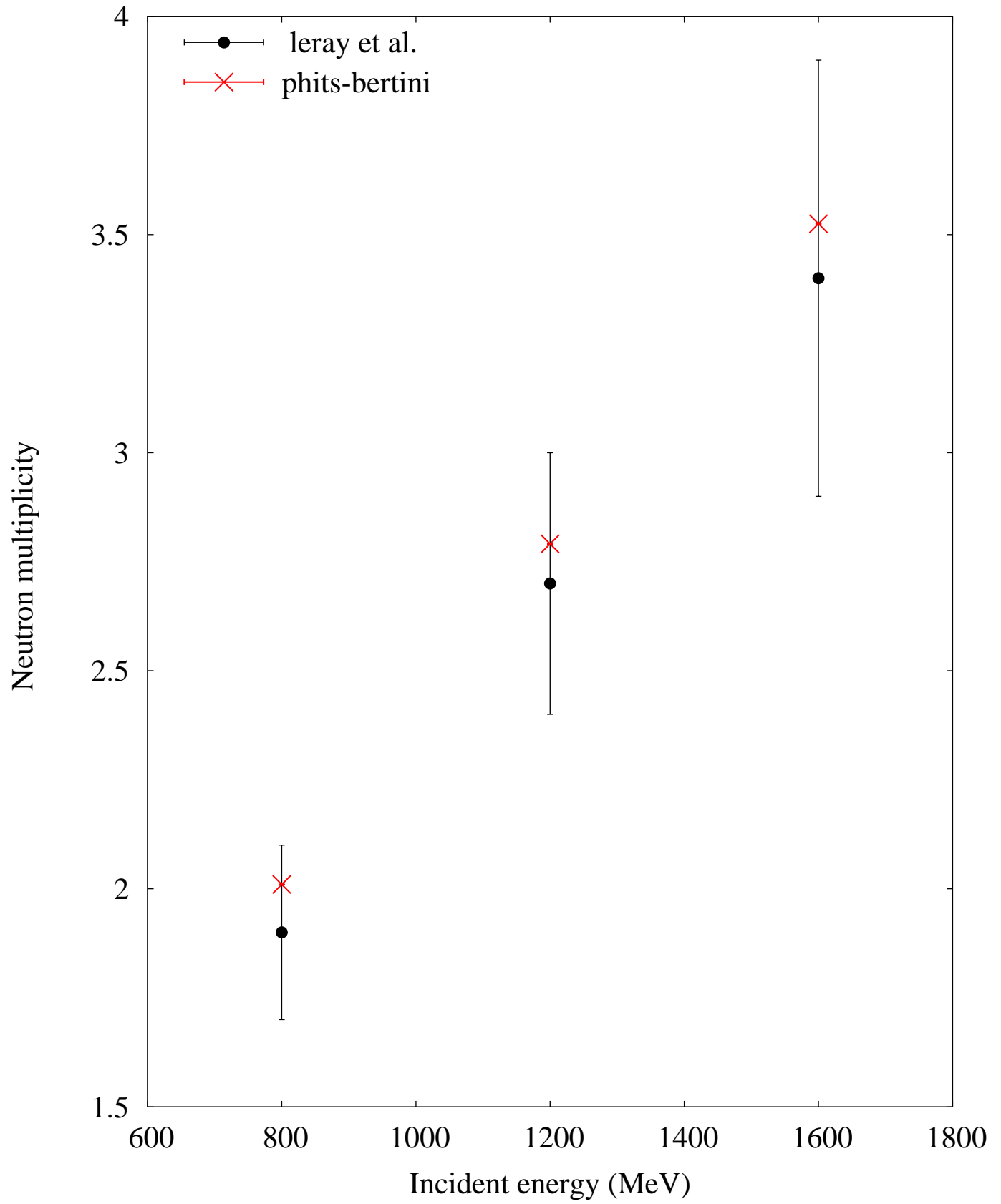
p + Pb -- (20+ MeV) Avg. neutron multiplicities
