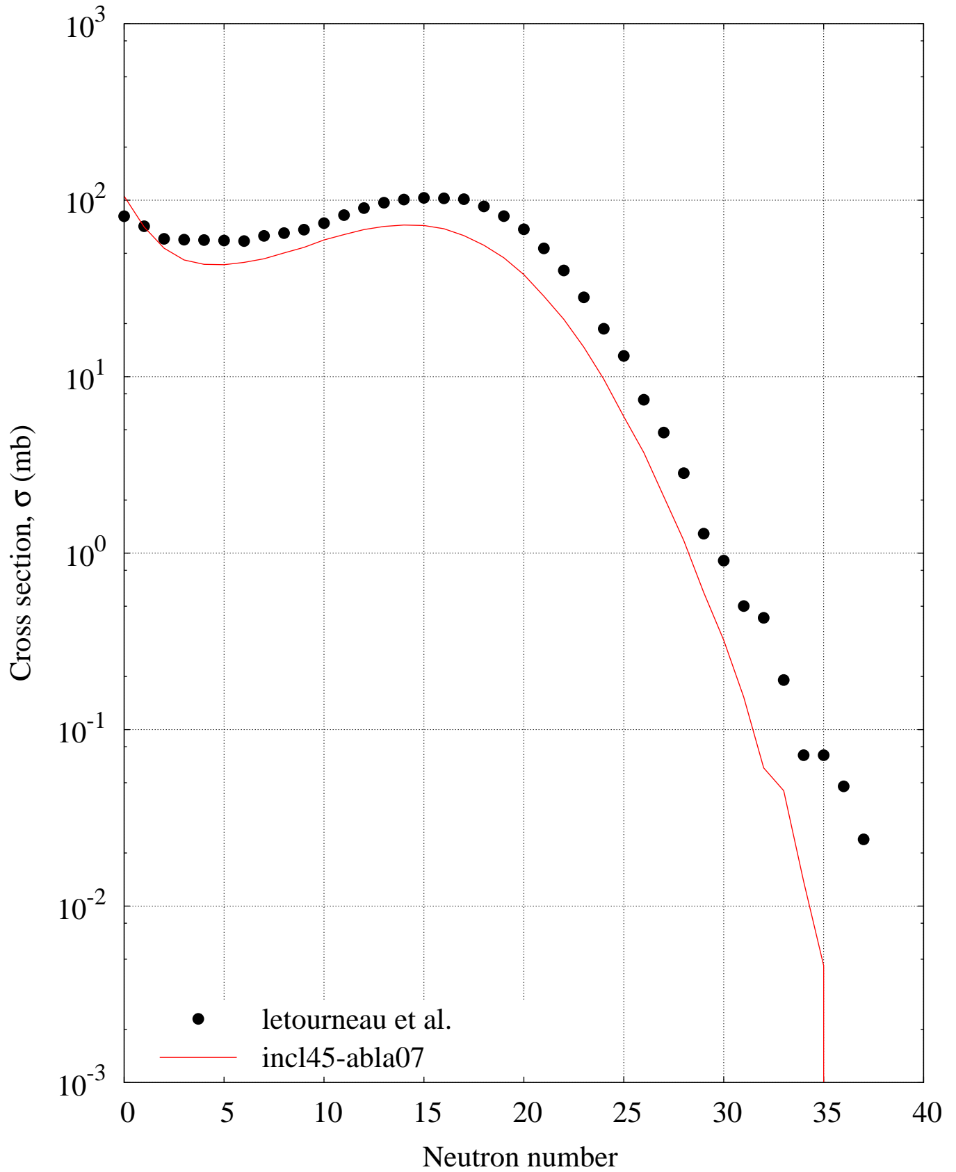
p (1200 MeV) + Pb -- Multiplicity distribution
