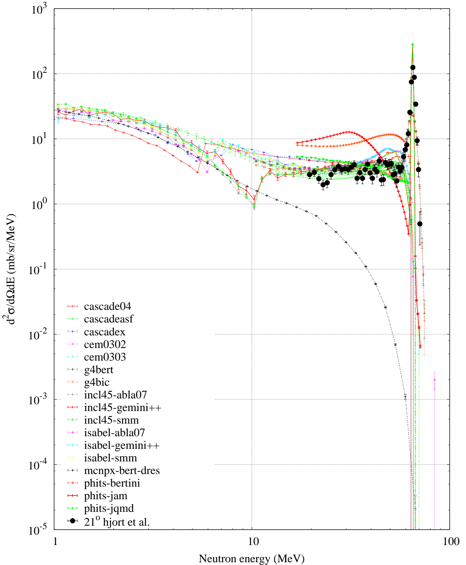
n (65 MeV) + Fe -- Neutron spectrum
