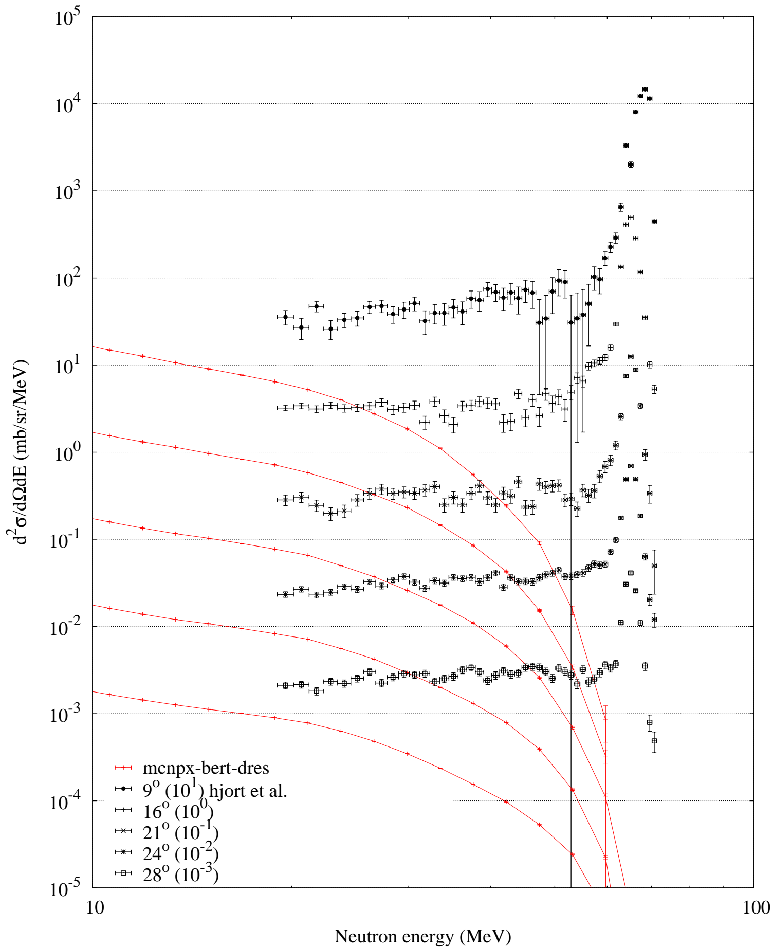
n (65 MeV) + Fe -- Neutron spectrum
