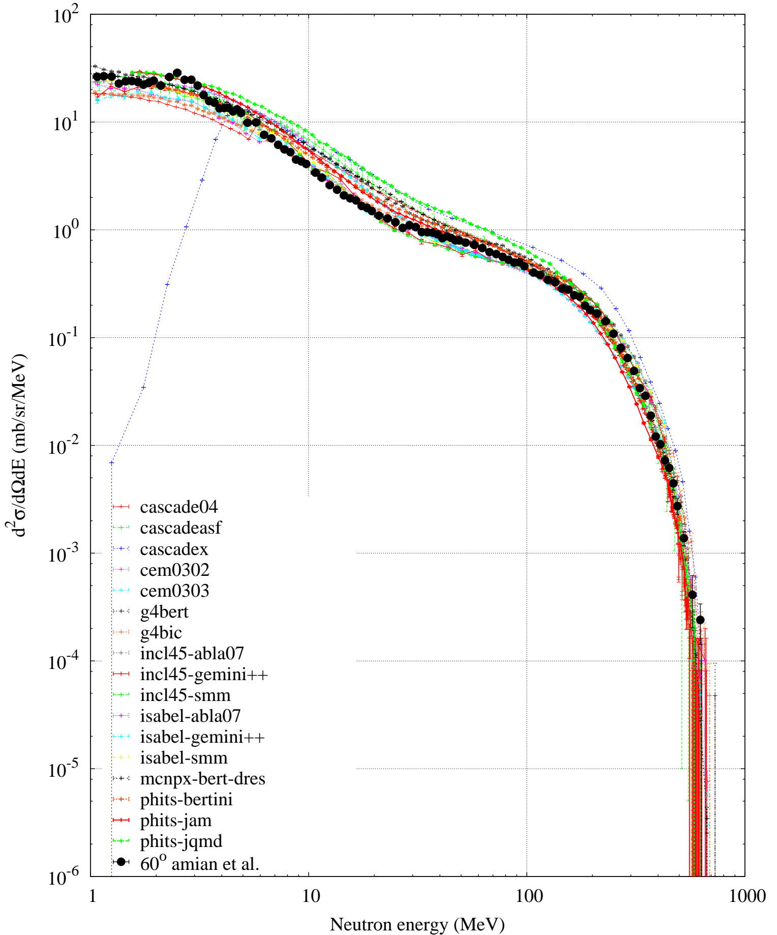
p (800 MeV) + Fe -- Neutron spectrum
