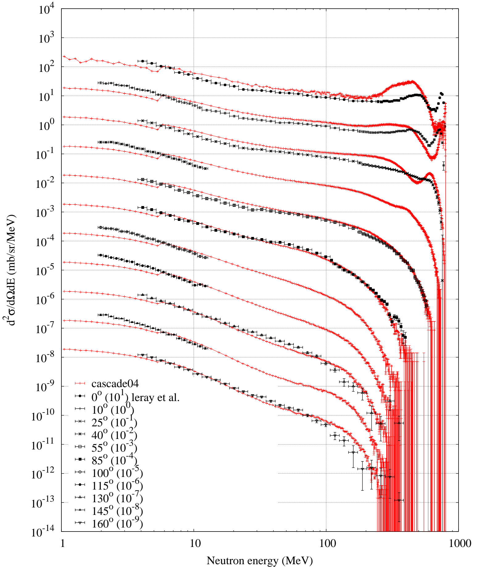
p (800 MeV) + Fe -- Neutron spectrum
