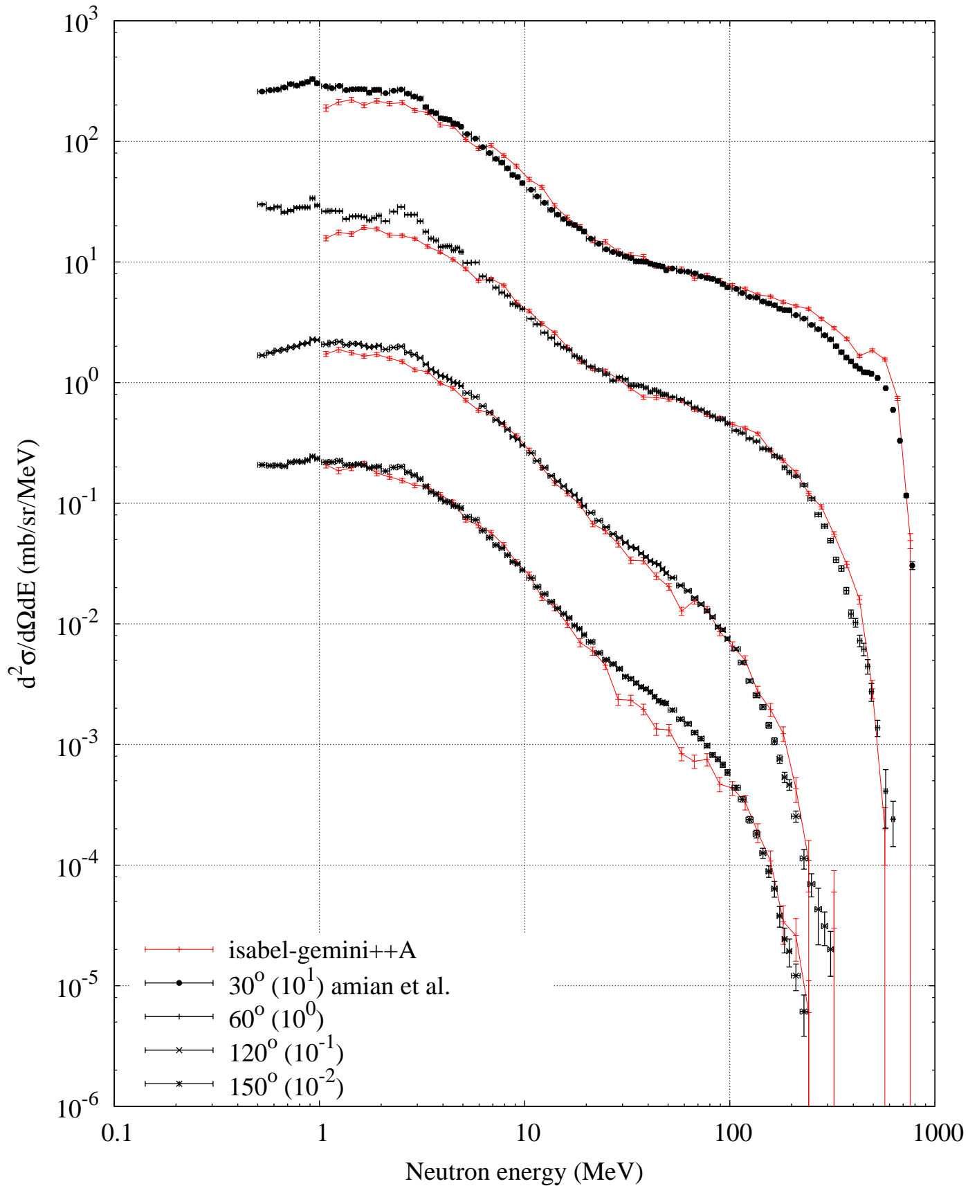
p (800 MeV) + Fe -- Neutron spectrum
