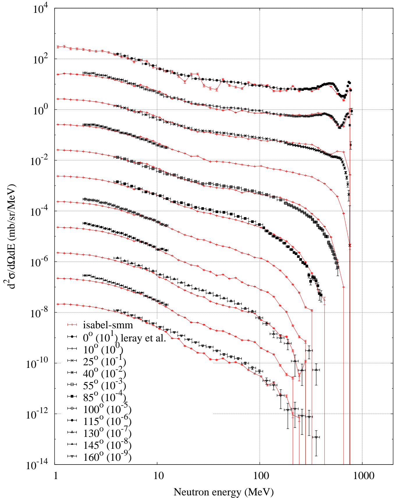
p (800 MeV) + Fe -- Neutron spectrum
