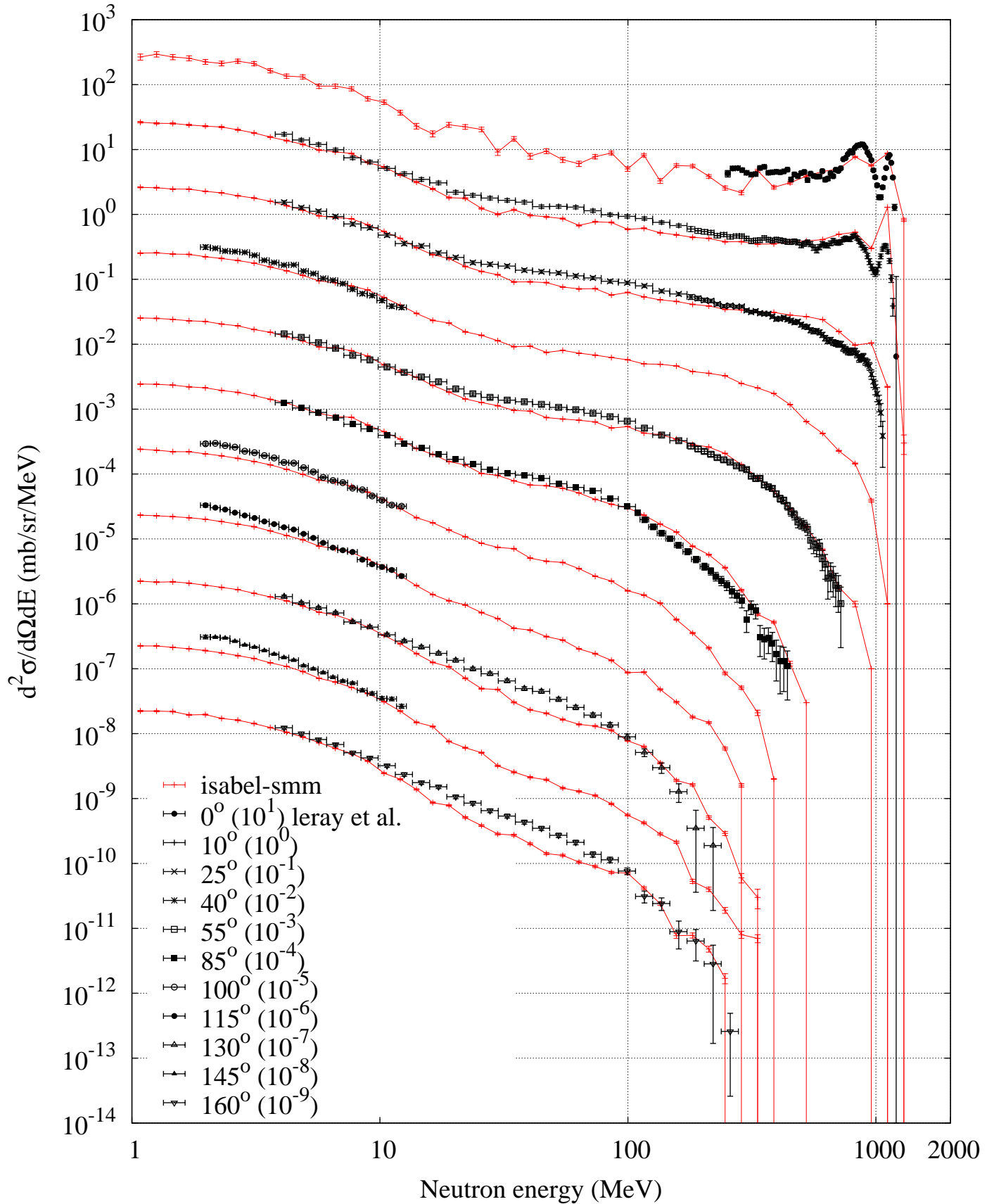
p (1200 MeV) + Fe -- Neutron spectrum
