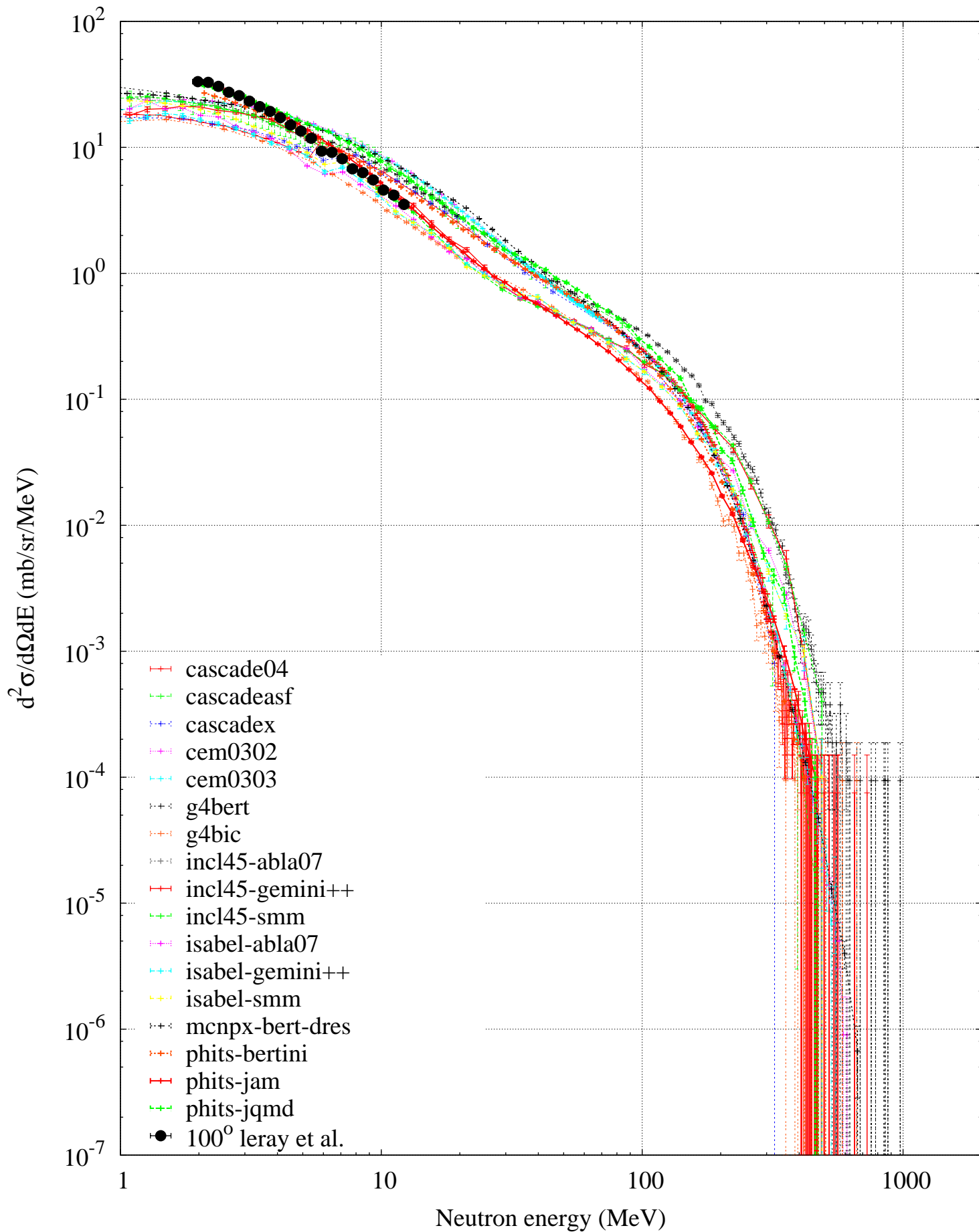
p (1600 MeV) + Fe -- Neutron spectrum
