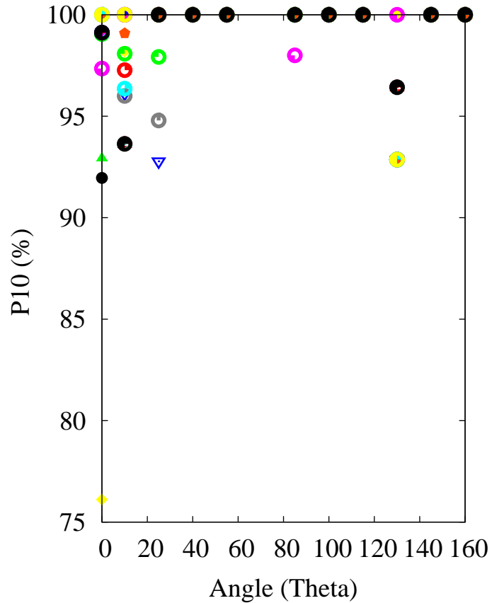
P10 factor - E_{\text{tot}} (full energy range)
