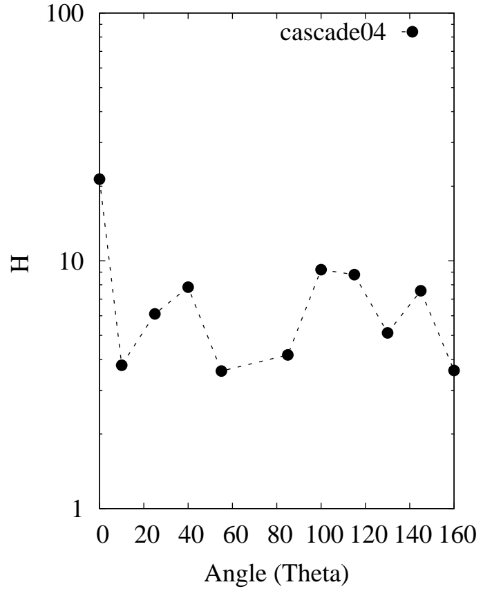
H factor - E_{\text{tot}} (full energy range)
