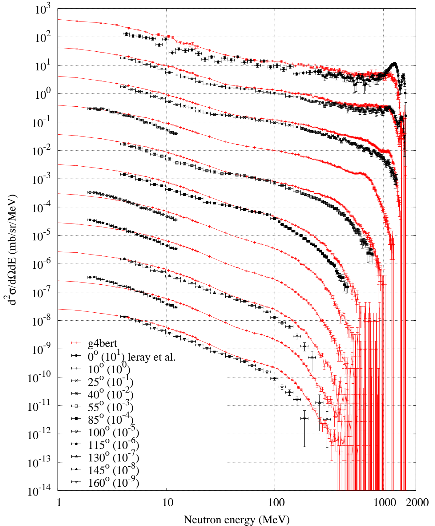
p (1600 MeV) + Fe -- Neutron spectrum
