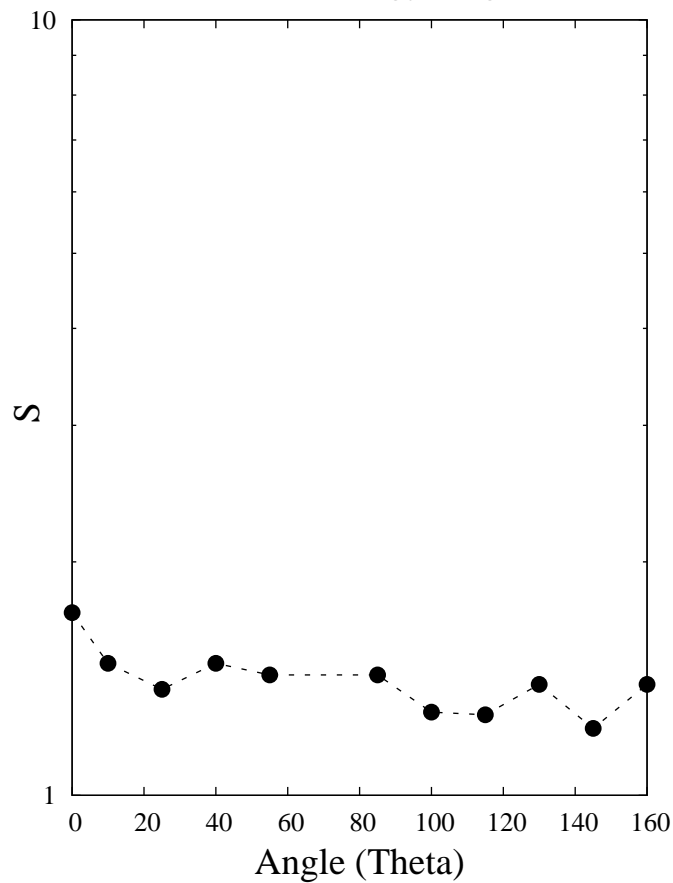
S factor - (Full energy range, MeV)
