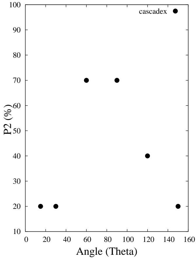
P2 factor - E_{\text{high}} (150+ MeV)
