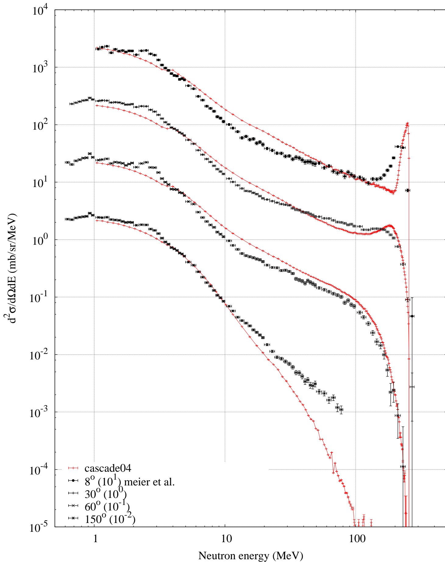
p (256 MeV) + Pb -- Neutron spectrum
