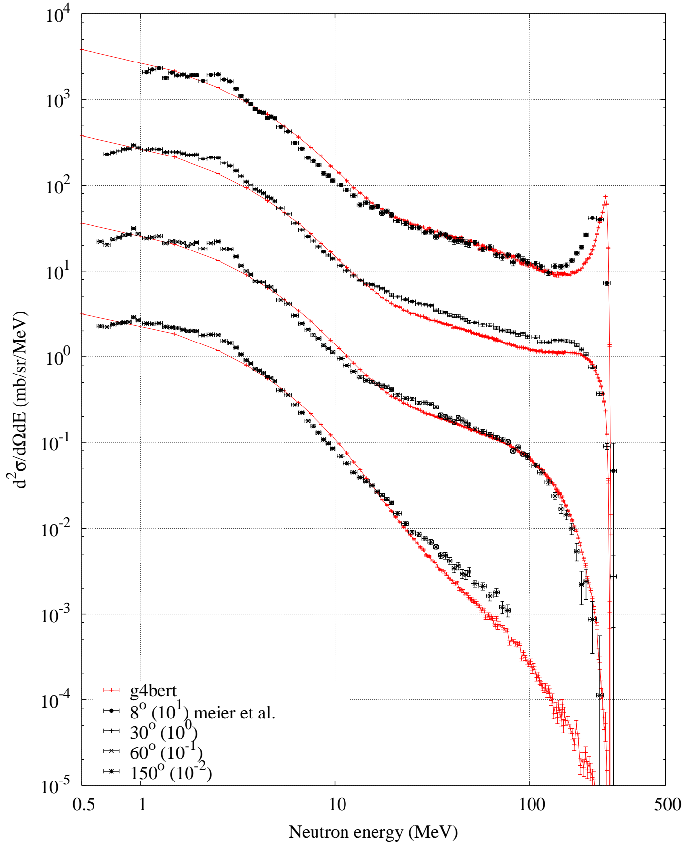
p (256 MeV) + Pb -- Neutron spectrum
