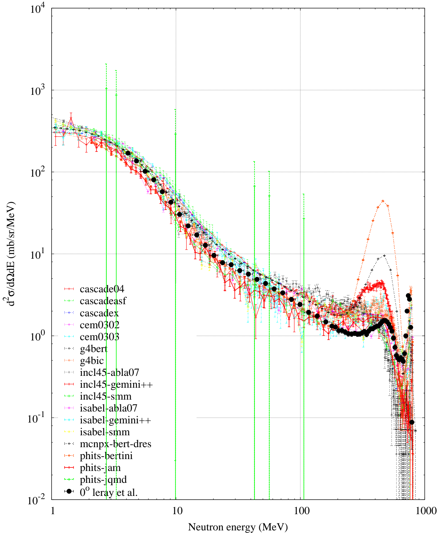
p (800 MeV) + Pb -- Neutron spectrum
