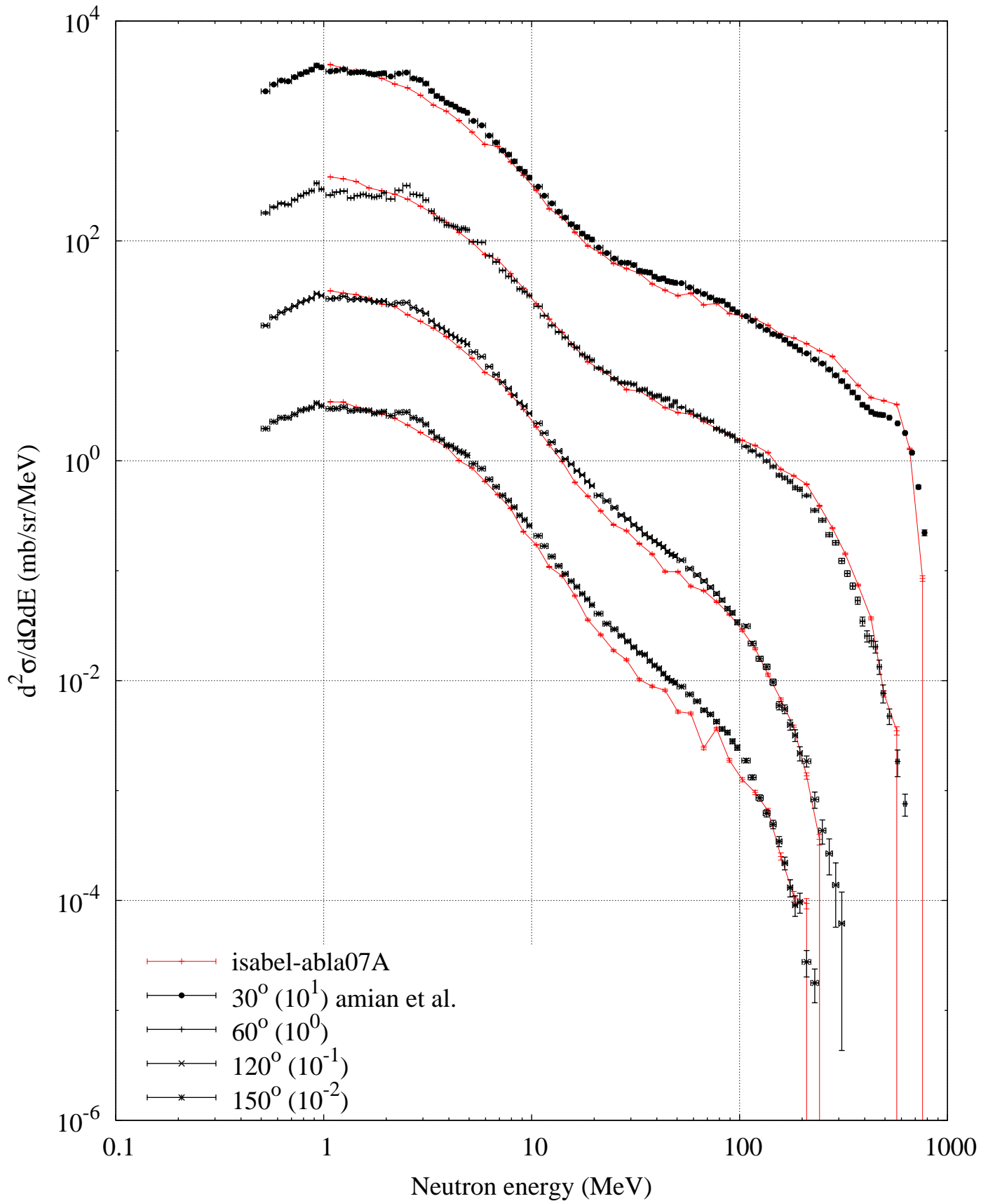
p (800 MeV) + Pb -- Neutron spectrum
