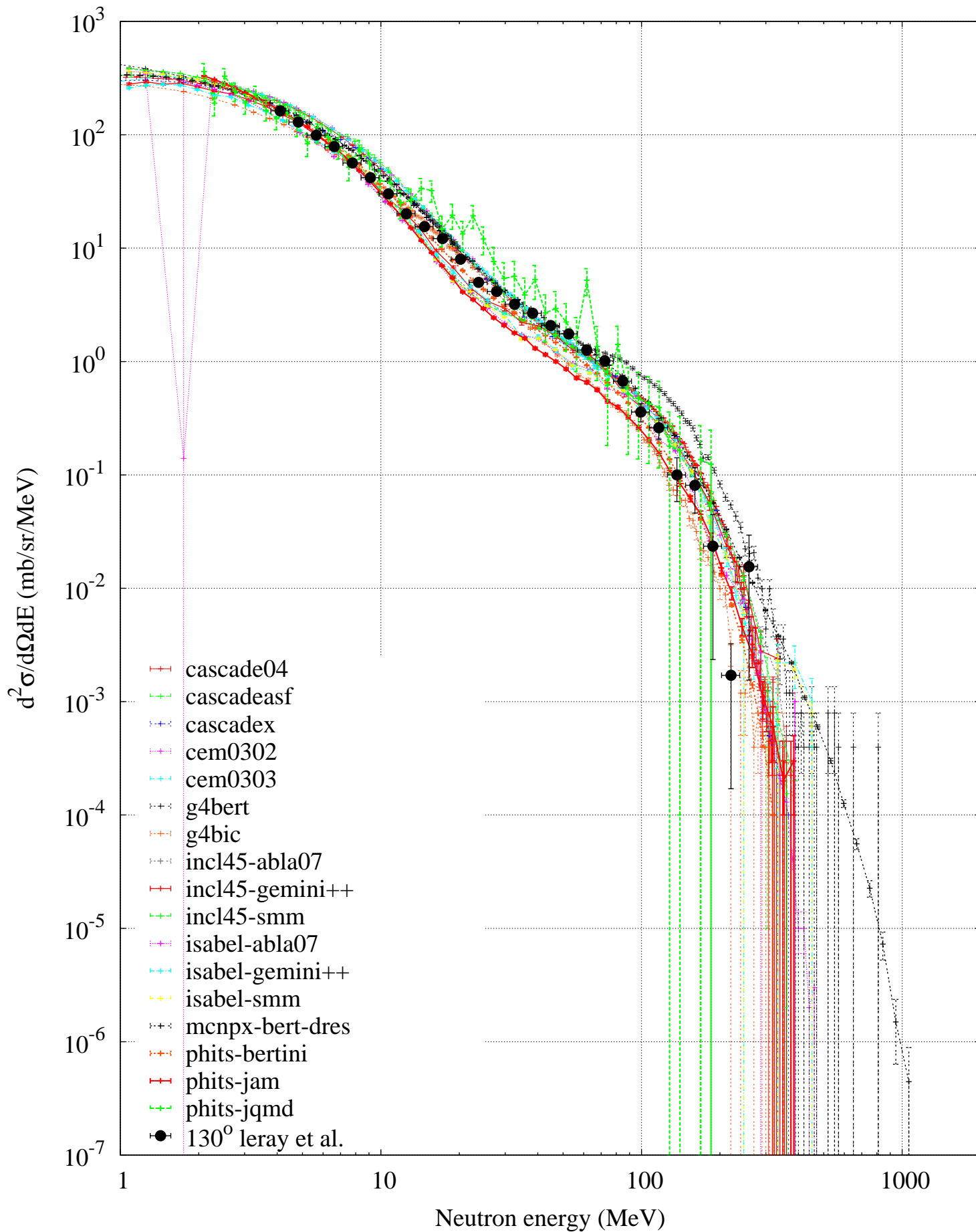
p (1200 MeV) + Pb -- Neutron spectrum
