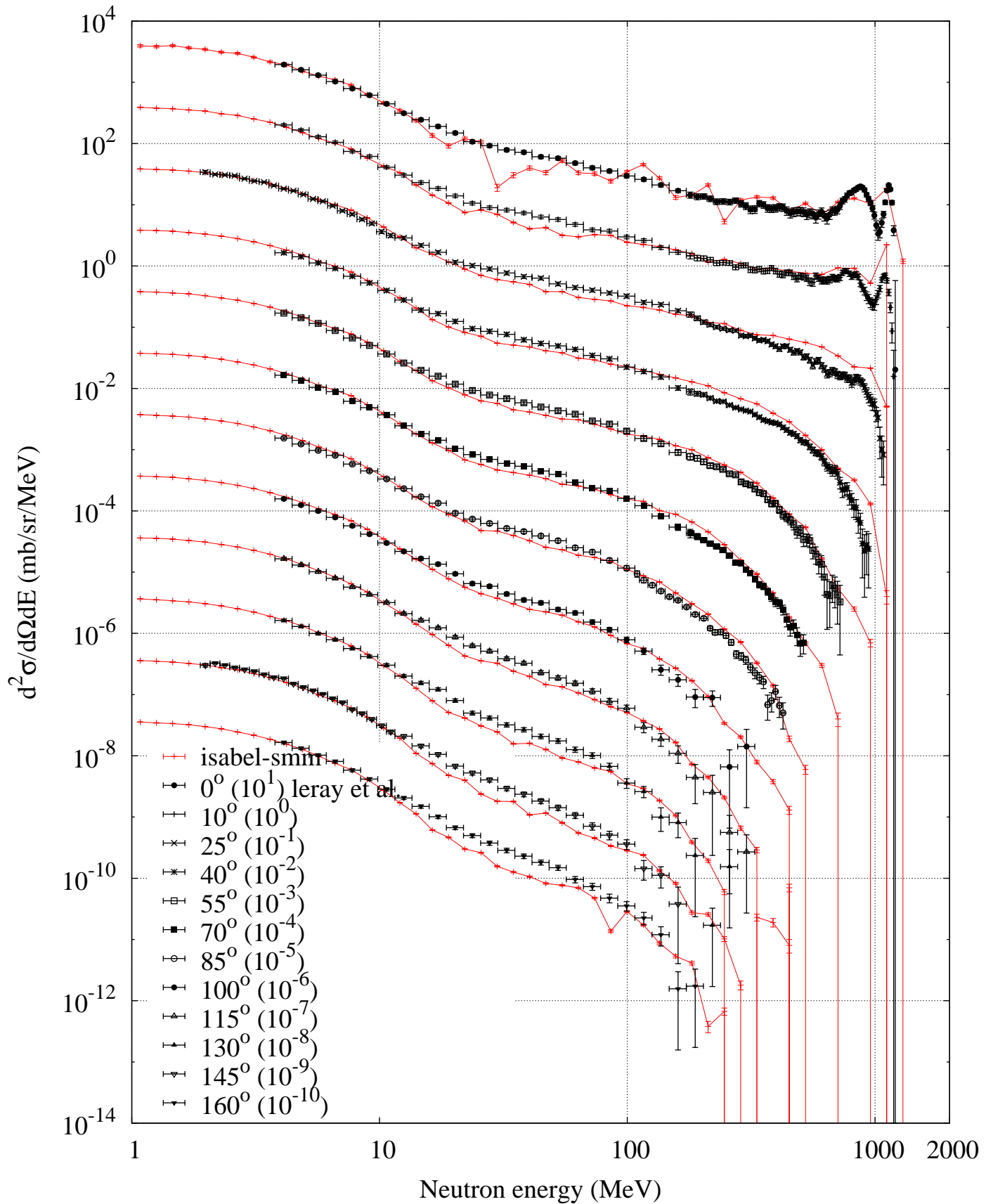
p (1200 MeV) + Pb -- Neutron spectrum
